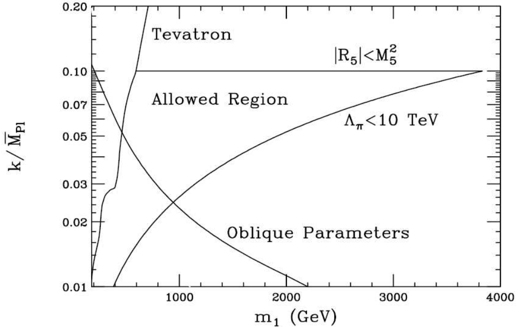
Figure 1.4: Summary of theoretical constraints on RS model [14]
