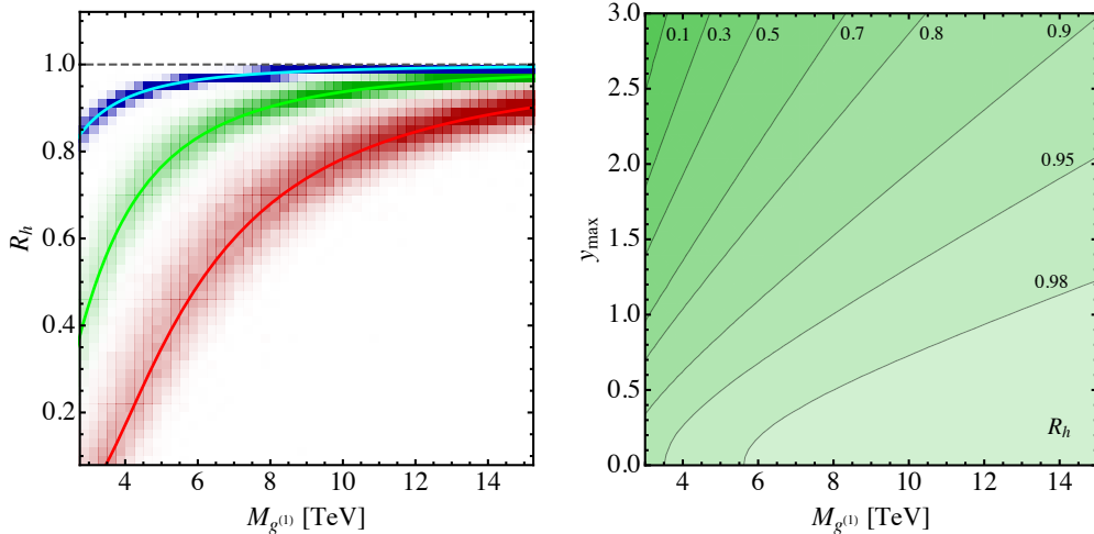
Figure 9.1: Predicted ratio R_h in a minimal RS model to the SM for \sigma(gg \rightarrow H) . The red, green, and blue density bands correspond to different choices of the parameter y_{\text{max}} (left). Contour plot of R_h using a parametrization of the center of the bands (right). [53]
