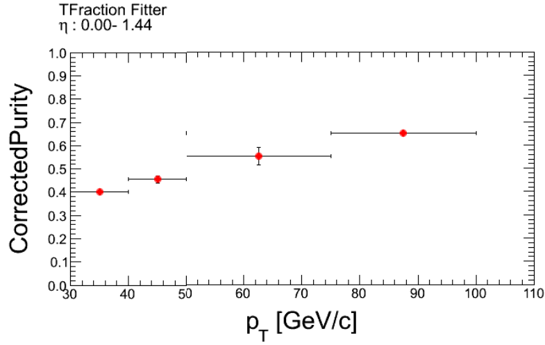
Figure 6.10: Corresponding Purity from TFraction Fitter
