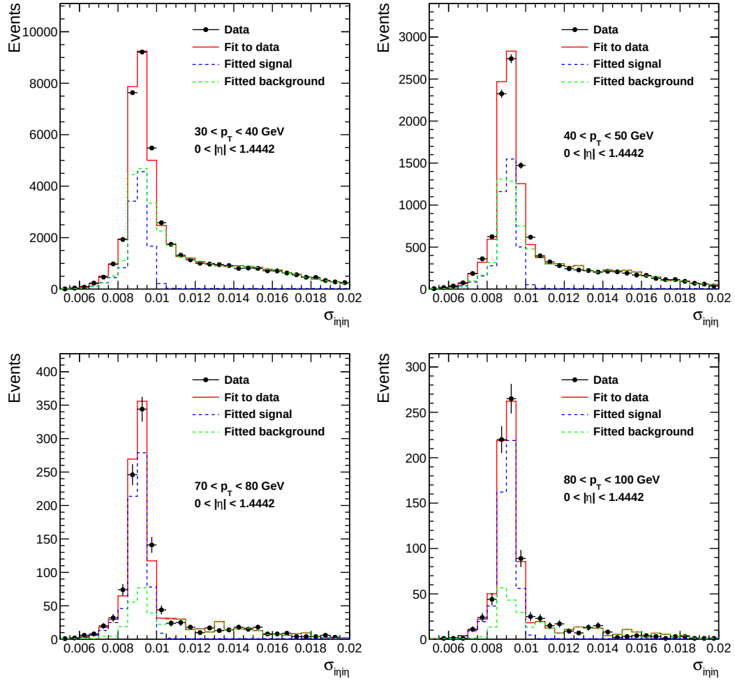
Figure 6.9: \sigma_{\eta\eta} template fits, in exclusive bins of p_T , in Jet trigger dataset. Note the sharper peak due to the photon template (blue lines), and the long tail for misidentified jets (green lines). The combined fit is shown in red, and the corresponding fractions are derived from the fit.
