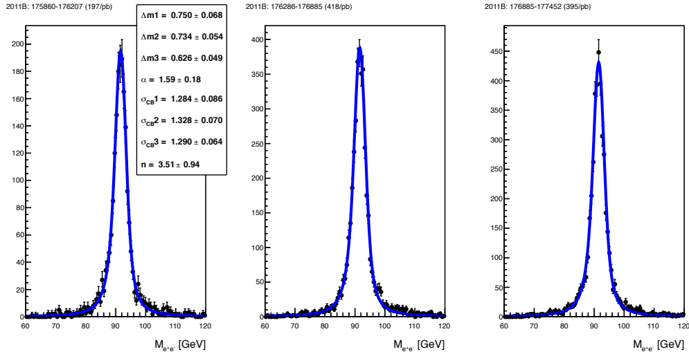
Figure C.2: \alpha and n floated, but shared
