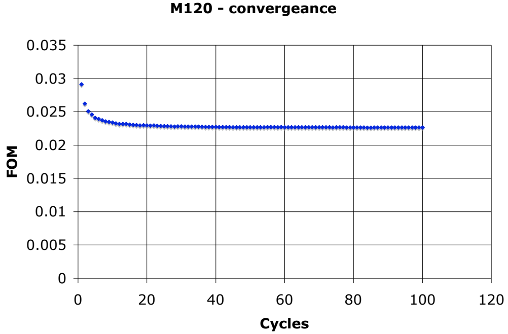
Figure A.7: Convergence of BDT training
