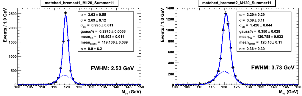
Figure B.13: Events selected by a cut at f(\text{brem}) > 2.0 (left) or < 2.0 (right) for the H \rightarrow \gamma\gamma Summer11 MC production. The reconstructed vertex was required to match the true vertex.
