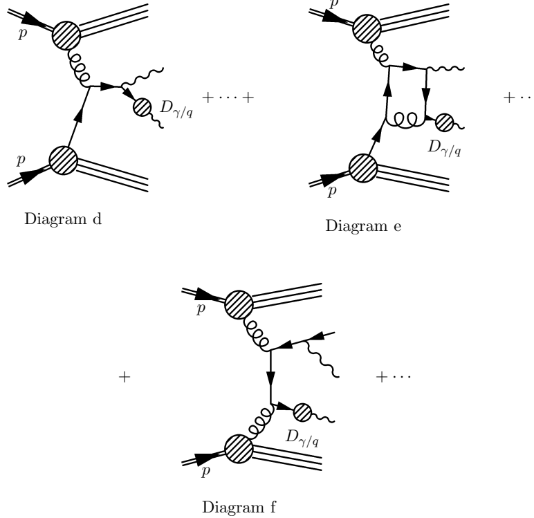
Figure 6.3: Single fragmentation diagrams. D: leading order fragmentation of a quark to photon. E: virtual gluon exchange correction to diagram D. F: same process replacing an initial state quark with a gluon [36].
