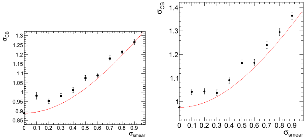
Figure B.20: Width of the signal peak for 110 GeV (left) and 120 GeV (right) H \rightarrow \gamma\gamma MC sample extracted with the fit, plotted vs. the injected smearing of the invariant mass.
