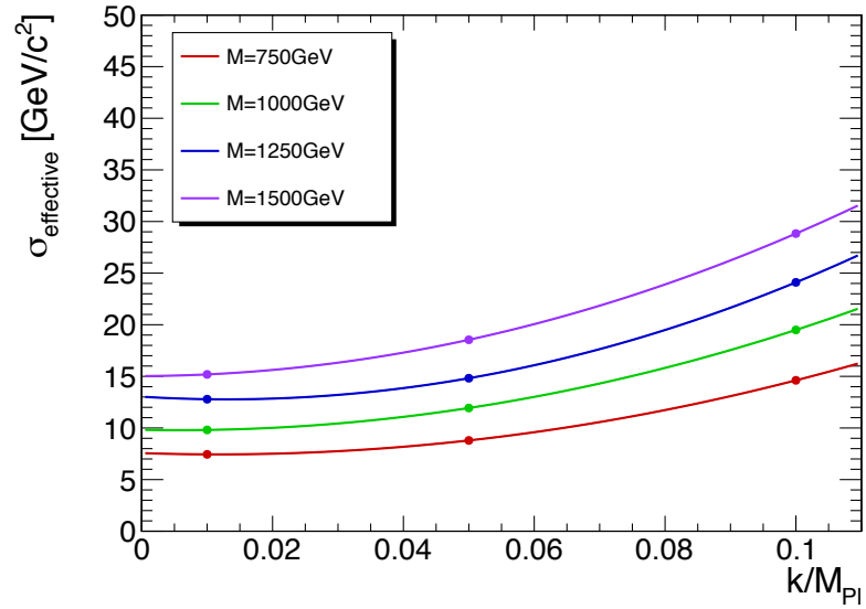
Figure 5.9: \sigma_{eff} for the RS graviton signal, as a function of \tilde{k} , for M_1 = 750, 1000, 1250, 1500 \text{ GeV}
