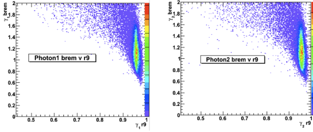
Figure B.10: Correlation between brem and R9.
