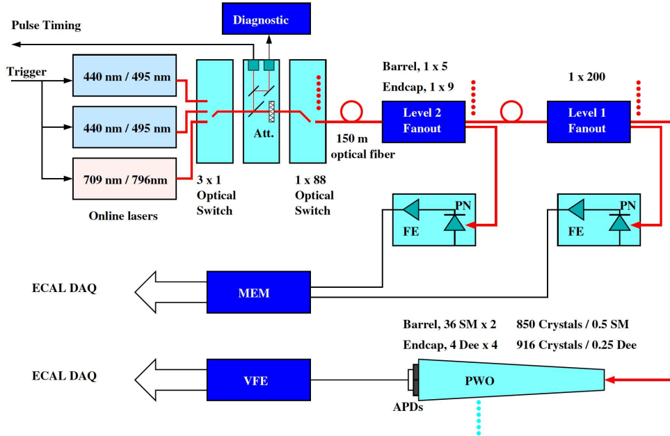
Figure 4.1: Diagram of Laser Monitoring Optical Components
