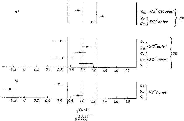
Fig. 6. Comparison of SU(3) couplings vs SU(6) predictions
