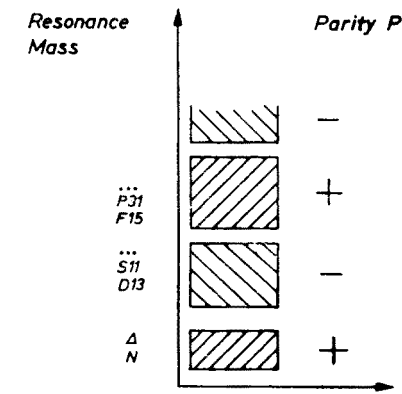
Fig. 1. Idealized view of the Baryon spectrum
