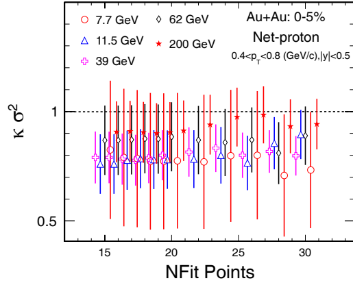
Figure 4.22: \kappa\sigma^2 of net-proton distributions as a function of number of fit points for Au+Au central collisions (0 – 5%) at \sqrt{s_{NN}} = 7.7, 11.5, 39, 62.4 and 200 GeV.
