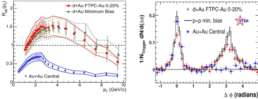
Figure 1.16: Left: R_{AB}(p_T) as a function of transverse momentum in d +Au and Au+Au 200 GeV collisions at RHIC. Right: Two particle azimuthal distributions in p+p, d +Au central and Au+Au central collisions at \sqrt{s_{NN}} = 200 GeV. The figures are taken from [55].
