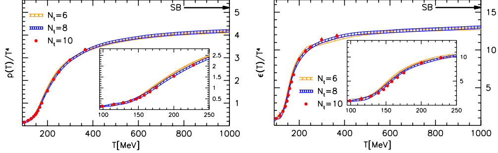
Figure 1.5: EOS in 2+1 flavor QCD with stout quarks at the physical point reported from Wuppertal-Budapest collaboration. The inset plots show the ratio of P/P_{SB} and \epsilon/\epsilon_{SB} , respectively. The figures are taken from [22].
