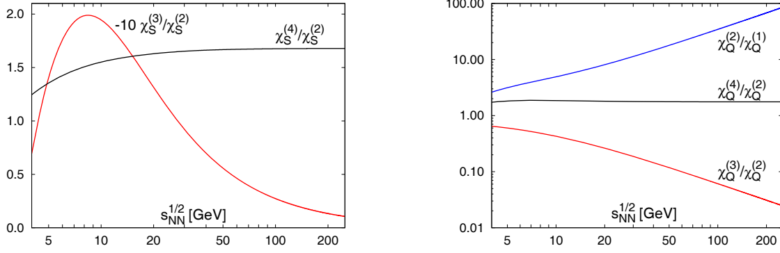
Figure 3.6: The ratios of moment products of strangeness and charge fluctuations along the chemical freeze-out curve, where the chemical potential and the temperature are parameterized as a function of colliding energy. The figures are taken from [58].
