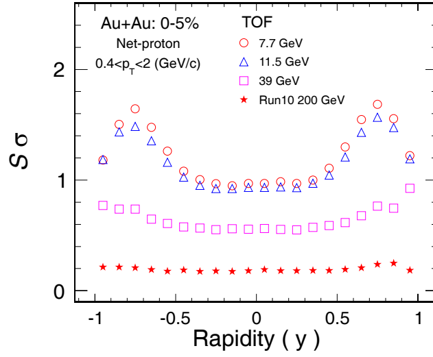
Figure 5.32: Differential rapidity dependence (interval \delta y = 0.1 ) of S\sigma for Au+Au central collisions at \sqrt{s_{NN}} = 7.7, 11.5, 39, 200 GeV (Run10).
