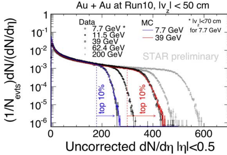
Figure 4.10: Comparison of refmult from 7.7 to 200 GeV at Run10. Note: |V_z| < 70 cm for 7.7 GeV. The blue and red are refmult distributions from Monte-Carlo simulation for 7.7 and 39 GeV, respectively.
