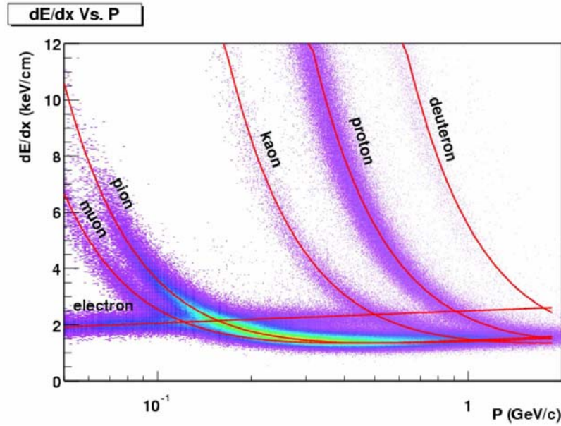
Figure 4.13: Particle identification with ionization energy loss ( dE/dx ), which is measured by STAR Time Projection Chamber (TPC). The solid lines in the figure are expectation line from bethe-bloch formula.
