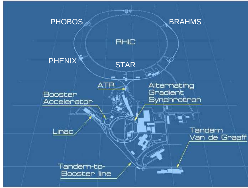
Figure 2.1: Schematic of the RHIC complex. Relativistic heavy ions collide at six intersection points along the RHIC ring of 3,814 m long.
