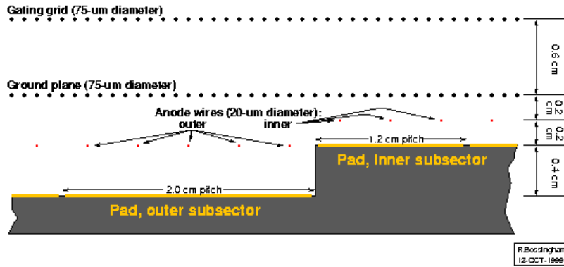
Figure 2.7: Cutaway view of wires relative to the inner and outer pad rows.
