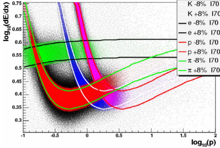
Figure 2.8: \log_{10}(dE/dx) (KeV/cm) as a function of \log_{10}(p) (GeV/c) for electron, pions, kaons and protons. The colored band are within the \pm 1\sigma dE/dx resolution. I70 denotes Bichsel's prediction for 30% truncated dE/dx mean [76].
