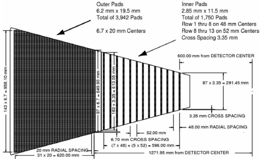
Figure 2.6: The anode pad plane of one full TPC sector. The inner sub-sector is on the right and it has small pads arranged in widely spaced rows. The outer sub-sector is on the left and it is densely packed with larger pads.
