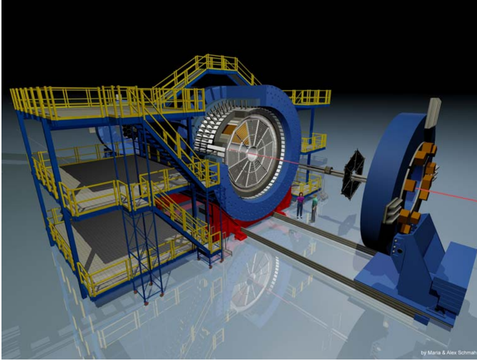
Figure 2.3: First 3D picture of the STAR detector. The figure is taken from [66].
