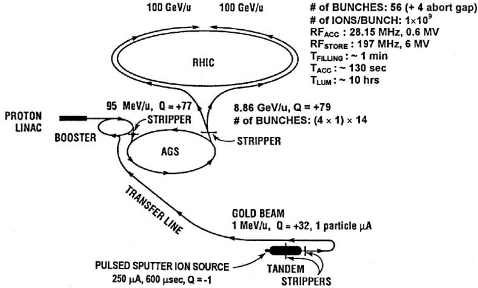
Figure 2.2: RHIC acceleration scenario for Au beam. The figure is taken from [64]
