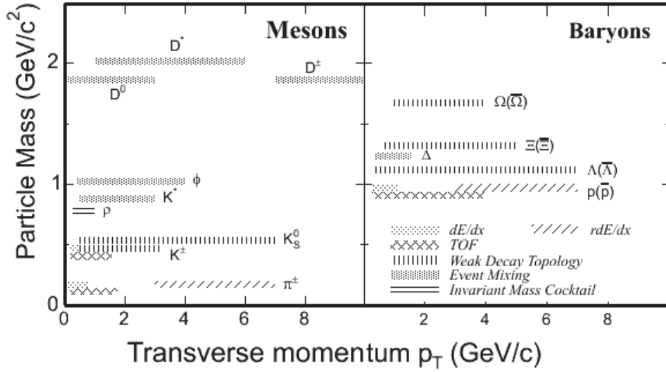
Figure 2.9: p_T reach of particle identification capability with STAR detectors. The upper edges of rdE/dx , weak decay topology, event mixing are limited by statistics. The figure is taken from [78].
