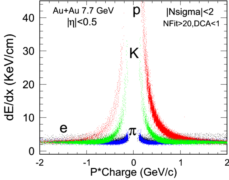
Figure 4.15: dE/dx versus rigidity for Au+Au collisions at \sqrt{s_{NN}}=7.7 GeV.
