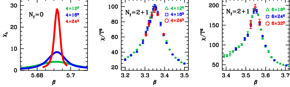
Figure 1.6: The volume dependence of the susceptibility peaks for pure SU(3) gauge theory (Polyakov-loop susceptibility, left panel) and for full QCD (chiral susceptibility on N_\tau=4 and 6 lattices, middle and right panels, respectively).
