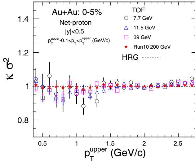
Figure 5.23: \kappa\sigma^2 as a function of differential p_T with TOF PID for Au+Au central collisions at \sqrt{s_{NN}} = 7.7, 11.5, 39, 200 GeV. The line in the figures is the HRG model calculations.
