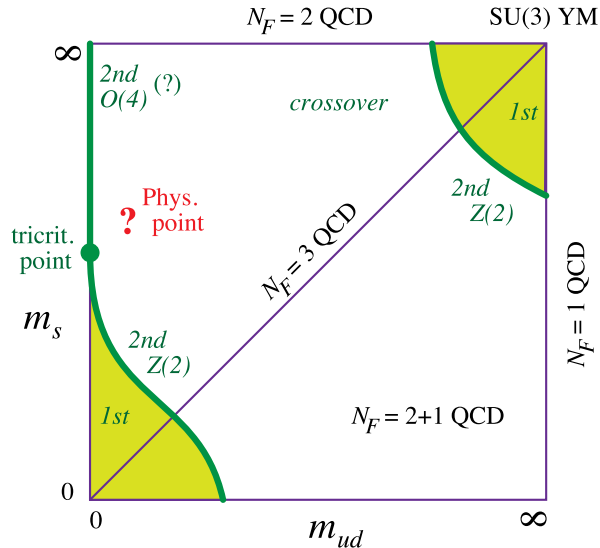
Figure 1.4: The Columbia-plot: the nature of the finite temperature transition in 2+1 flavor QCD at \mu_B = 0 as a function of the degenerate u and d quark mass m_{ud} and the s quark mass m_s . The figure is taken from [21].
