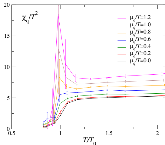
Figure 1.7: Quark number susceptibility as a function of temperature and \mu_q/T by a simulation with an improved Wilson quark action. T_0 is T_c at \mu_q = 0 . The figure is taken from [23].
