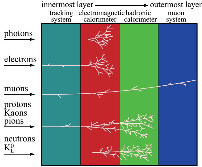
Figure 4.11: Illustration of particle identification by interaction pattern. The figure is taken from [106].
