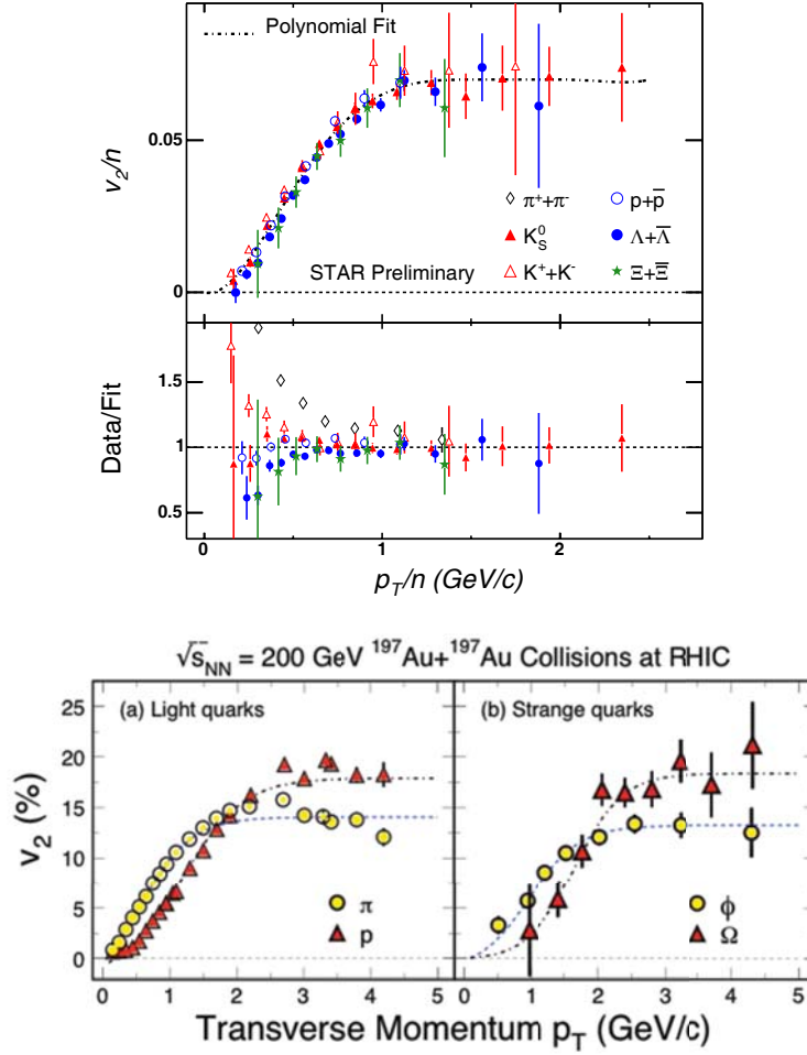
Figure 1.15: Upper panel: Test of number of quarks (NQ) scaling of identified hadron v_2 in Au+Au minimum-bias collisions at \sqrt{s_{NN}} = 200 GeV (The lower plot shows the ratio of the data to the dashed-dotted fit to the data in the upper plot.) Lower panel: v_2 as a function of p_T for \pi , p (left) and \phi , \Omega (right). Lines represent NQ-inspired fit. The figures are taken from [50, 52].
