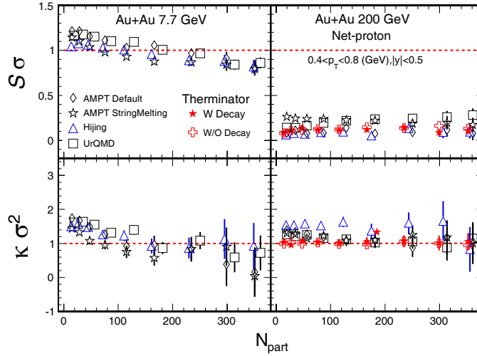
Figure 3.9: Centrality dependence of S\sigma and \kappa\sigma^2 of net-proton distributions for Au+Au collisions at \sqrt{s_{NN}} = 7.7, 200 GeV from various models.
