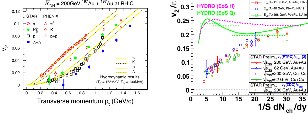
Figure 1.14: Left Panel : Elliptic flow v_2 for different particle species measured by STAR and PHENIX compared to hydrodynamic model predictions. The data indicates the expected mass ordering in this low p_T region. Right Panel : Compilation of v_2/\epsilon for charged hadrons as a function of particle density at mid-rapidity. Green dashed lines represent ideal hydrodynamic limit for AGS, SPS and RHIC collision energies. The figures are taken from [50, 51].
