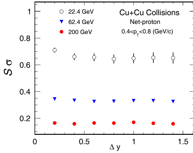
Figure 5.27: Rapidity window size dependence of S\sigma for Cu+Cu central collisions (0 – 10%, 22.4 GeV: 0 – 5%) at \sqrt{s_{NN}} = 22.4, 62.4, 200 GeV.
