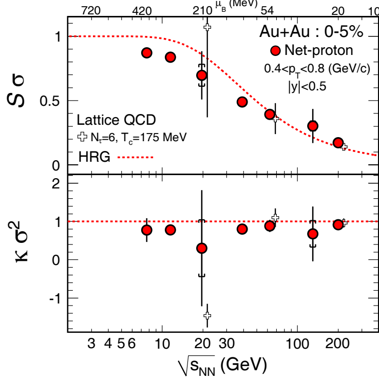
Figure 5.6: Energy dependence of moment products ( \kappa\sigma^2 and S\sigma ) of net-proton distributions for central Au+Au collisions (0 – 5%, 19.6 GeV: 0 – 10%, 130 GeV: 0 – 6%). The red dashed lines denote the HRG model calculations, in which the S\sigma = \tanh(\mu_B/T) and \kappa\sigma^2=1 . The empty markers denote the results calculated from Lattice QCD.
