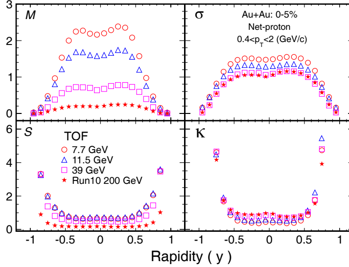
Figure 5.31: Various Moments ( M, \sigma, S, \kappa ) of net-proton distributions as a function of differential rapidity ( \delta y = 0.1 ) with TOF PID for Au+Au central collisions at \sqrt{s_{\text{NN}}} = 7.7, 11.5, 39, 200 GeV (Run10).
