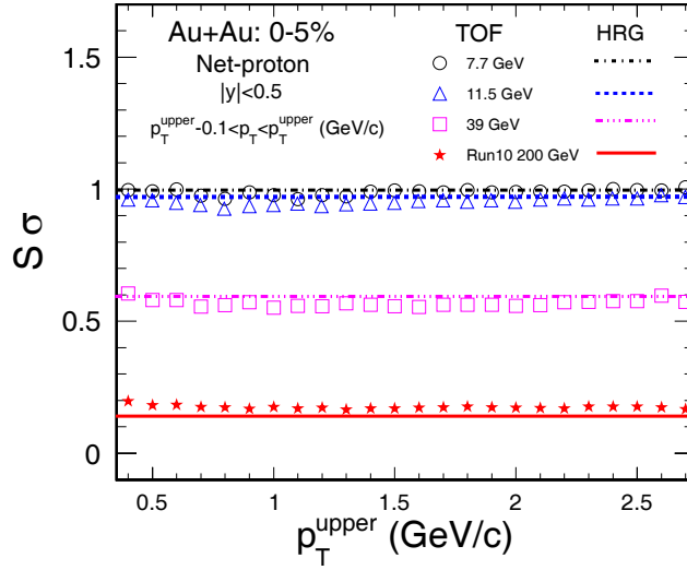
Figure 5.22: S\sigma as a function of differential p_T with TOF PID for Au+Au central collisions at \sqrt{s_{NN}} = 7.7, 11.5, 39, 200 GeV. The lines in the figures are HRG model calculations for each energy.
