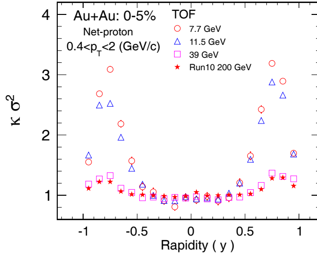
Figure 5.33: Differential rapidity dependence (interval \delta y = 0.1 ) of \kappa\sigma^2 for Au+Au central collisions at \sqrt{s_{NN}} = 7.7, 11.5, 39, 200 GeV (Run10).
