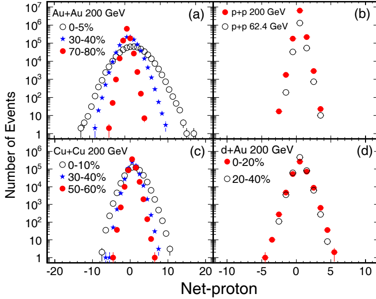
Figure 5.1: Typical event-by-event net-proton multiplicity distributions for p+p, d+Au, Cu+Cu and Au+Au collisions.
