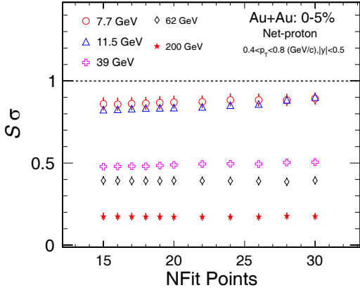
Figure 4.21: S\sigma of net-proton distributions as a function of number of fit points for Au+Au central collisions (0 – 5%) at \sqrt{s_{NN}} = 7.7, 11.5, 39, 62.4 and 200 GeV.
