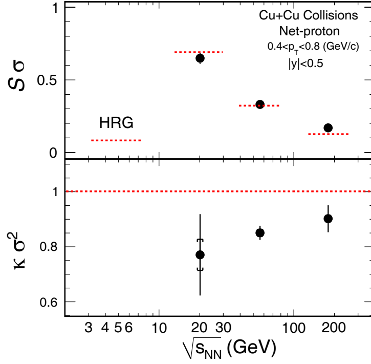
Figure 5.9: Energy dependence of moment products ( \kappa\sigma^2 and S\sigma ) of net-proton distributions for Cu+Cu central collisions (0 – 10%, 22.4 GeV: 0 – 5%). The dashed lines shown in the figures are from HRG model calculations, in which S\sigma = \tanh(\mu_B/T) and \kappa\sigma^2=1 .
