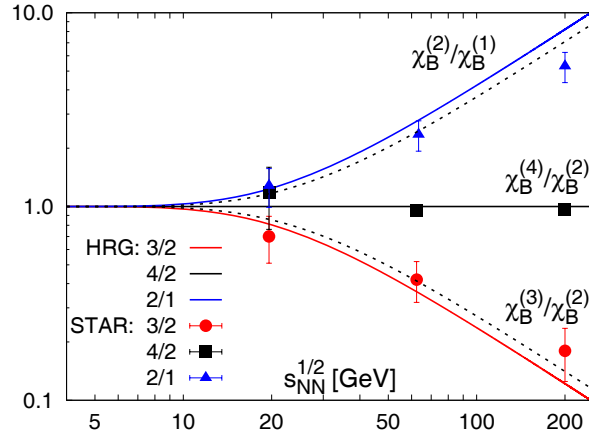
Figure 3.5: The ratio of quadratic fluctuations and mean net-baryon number ((\sigma^2/M)_B) , cubic to quadratic ((S\sigma)_B) and quartic to quadratic ((\kappa\sigma^2)_B) baryon number fluctuations calculated in the HRG model on the freeze-out curve and compared to results obtained by the STAR collaboration. The dashed curves show the approximate results for (\kappa\sigma^2)_B = 1 and (S\sigma)_B = \tanh(\mu_B/T) , respectively. The figure is taken from [58].
