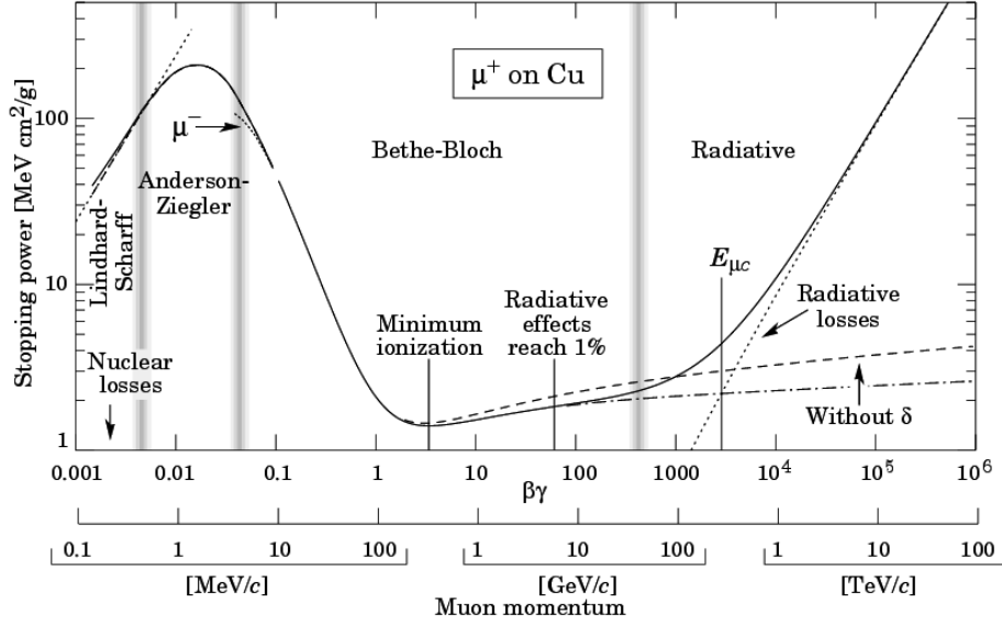
Figure 4.12: Ionization Energy Loss of \mu^+ in copper. The figure is taken from [107].
