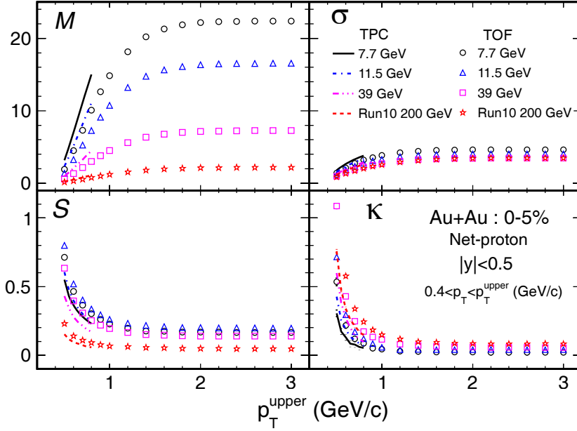
Figure 5.18: Various moments ( M, \sigma, S, \kappa ) of net-proton distributions with TPC (lines) and TOF PID as a function of p_T coverage for Run 10 Au+Au central collisions at \sqrt{s_{NN}} = 7.7, 11.5, 39 and 200 GeV.
