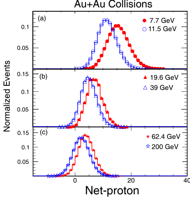
Figure 5.2: Typical event-by-event net-proton multiplicity distributions for Au+Au central collisions at \sqrt{s_{NN}} = 7.7, 11.5, 39, 62.4, 200 GeV.
