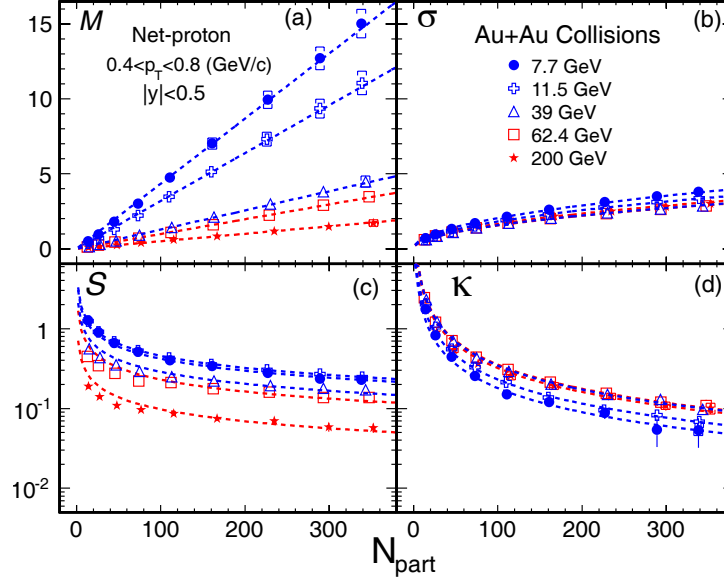
Figure 5.3: Centrality dependence of various moments of net-proton multiplicity distributions for Au+Au collisions at \sqrt{s_{NN}} = 7.7, 11.5, 39, 62.4, 200 GeV. The dash lines shown in the figure are expectation lines from Central Limit Theorem (CLT).
