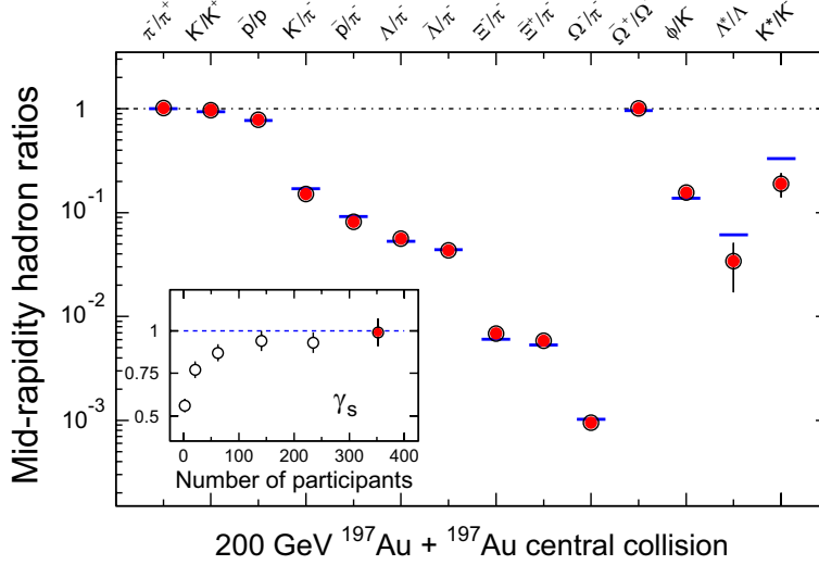
Figure 1.11: Ratios of p_T -integrated mid-rapidity yields for different hadron species measured in STAR for central Au+Au collisions at \sqrt{s_{NN}} = 200 GeV. The horizontal bars represent thermal model fits to the measured yield ratios for stable and long-lived hadrons. The variation of \gamma_s with centrality is shown in the inset, including the value (leftmost point) from fits to yield ratios measured by STAR for 200 GeV p+p collisions. The figure is taken from [45].
