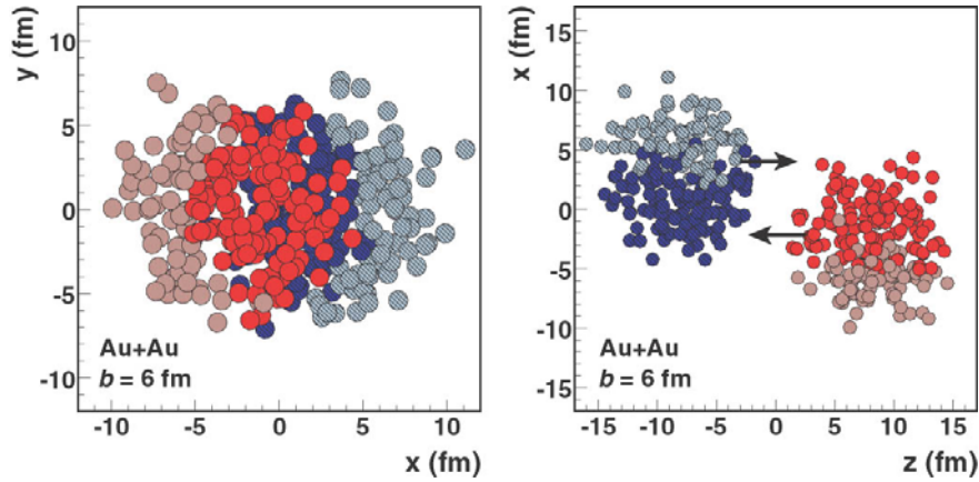
Figure 4.7: Illustration of a Glauber Monte Carlo event for Au+Au at \sqrt{s_{NN}} = 200 GeV with impact parameter b = 6 fm in the transverse plane (left panel) and along the beam axis (right panel). The nucleons are drawn with a radius \sqrt{\sigma_{inel}^{NN}/\pi}/2 . Darker disks represent participating nucleons. The figures are taken from [104].
