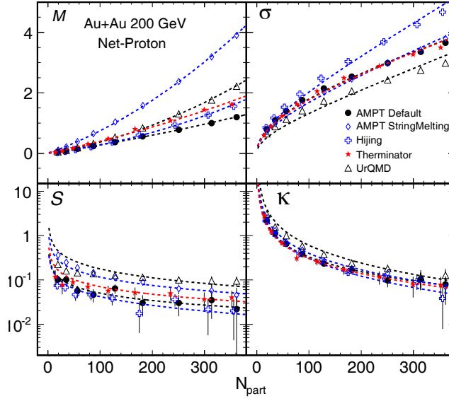
Figure 3.8: Centrality dependence of various moments of net-proton distributions for Au+Au collisions at \sqrt{s_{NN}} = 200 GeV from various models.
