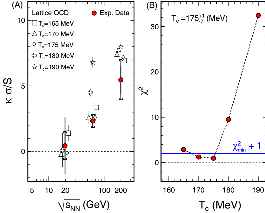
Figure 5.14: Comparison of \kappa\sigma/S from experiment and lattice predictions, and the extraction of T_c . (A): \kappa\sigma/S of net-proton distribution measured in collisions of Au ions at varying \sqrt{s_{NN}} and with an impact parameter of less than 3 fm. This is compared to lattice QCD predictions with cutoff 1/a \simeq 960 - 1000 MeV for the corresponding ratio of susceptibilities extrapolated to the freeze-out conditions using different values of T_c . The lattice results at each \sqrt{s_{NN}} are slightly shifted for clarity in presentation. (B): The comparison of experimental data and lattice QCD predictions, shown through \chi^2 as a function of T_c using the definition given in Equ. 5.3. This yields the estimate of T_c and its errors as discussed in the text.
