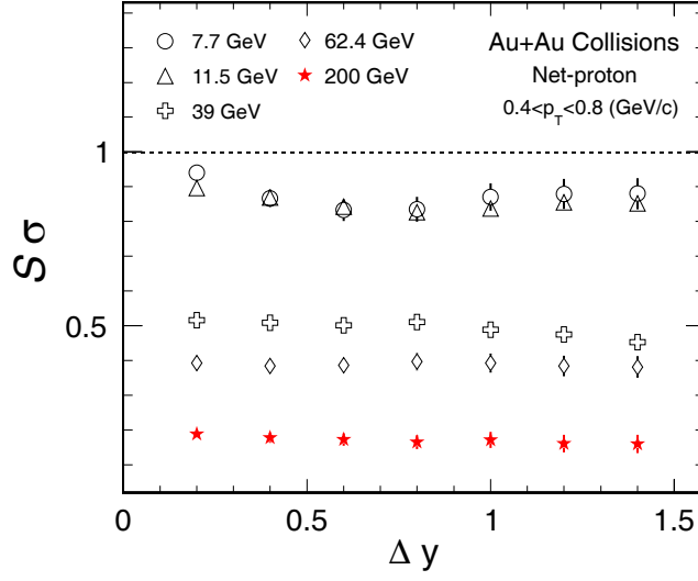
Figure 5.25: Rapidity window size dependence of S\sigma for Au+Au central collisions (0 – 5%) at \sqrt{s_{\text{NN}}} = 7.7, 11.5, 39, 62.4 and 200 GeV.
