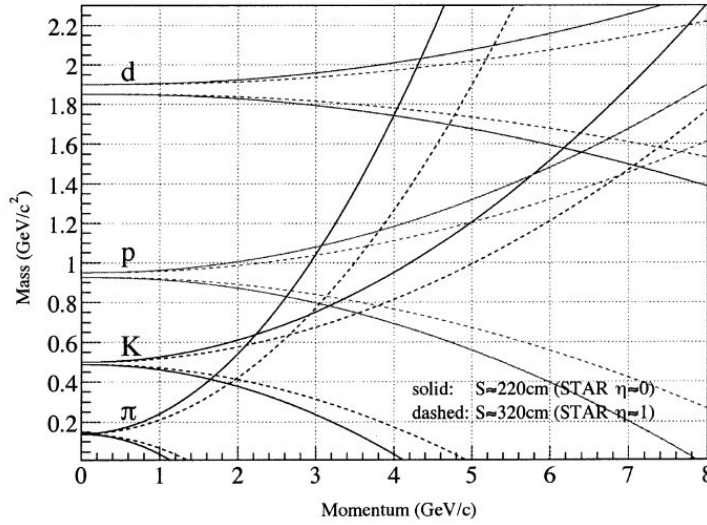
Figure 4.17: The momentum dependence of the particle identification capabilities of a TOF system with a timing resolution of 100 ps in the STAR geometry and with the STAR TPC's resolution on the track momentum and path length. The figure is taken from [84].
