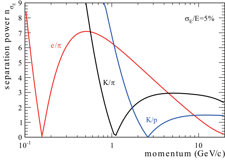
Figure 4.14: Separation power with TPC dE/dx particle identification.
