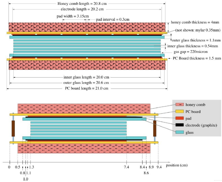
Figure 2.12: Two side-view of a MRPC moduel. The figure is taken from [85].
