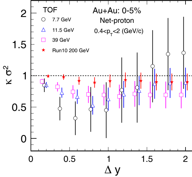
Figure 5.30: Rapidity window size dependence of \kappa\sigma^2 of net-proton distributions with TOF PID for Au+Au central collisions (0 – 5%) at \sqrt{s_{NN}} = 7.7, 11.5, 39 and Run10 200 GeV.
