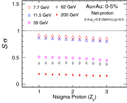
Figure 4.23: S\sigma of net-proton distributions as a function of Nsigma Proton ( Z_p ) for Au+Au central collisions (0 – 5%) at \sqrt{s_{NN}} = 7.7, 11.5, 39, 62.4 and 200 GeV.
