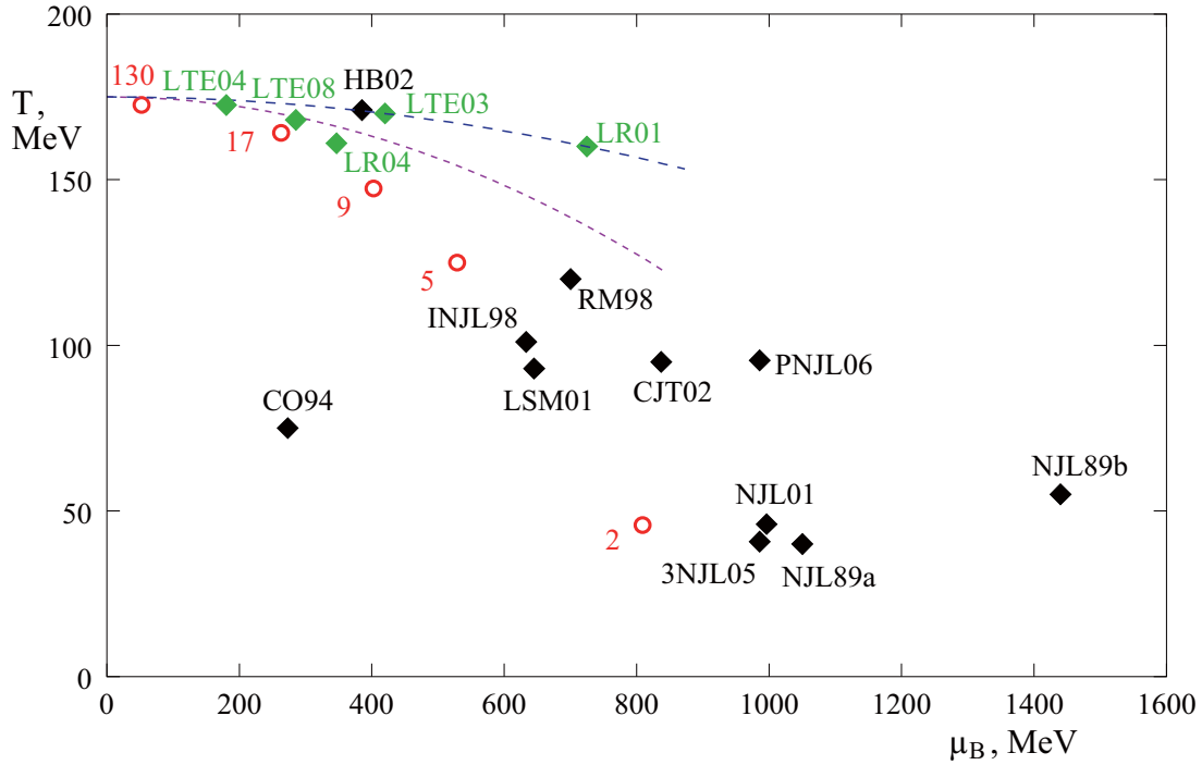
Figure 1.8: Comparison of predictions for the location of the QCD critical point on the phase diagram. Black points are model predictions: NJLa89, NJLb89 – [27], CO94 – [28, 29], INJL98 – [30], RM98 – [31], LSM01, NJL01 – [32], HB02 – [33], CJT02 – [34], 3NJL05 – [35], PNJL06 – [36]. Green points are lattice predictions: LR01, LR04 – [18, 37], LTE03 – [38], LTE04 – [39], LTE08 – [40]. The two dashed lines are parabolas with slopes corresponding to lattice predictions of the slope dT/d\mu_B^2 of the transition line at \mu_B = 0 [38, 41]. The red circles are locations of the freezeout points for heavy ion collisions at corresponding center of mass energies per nucleon (indicated by labels in GeV).
