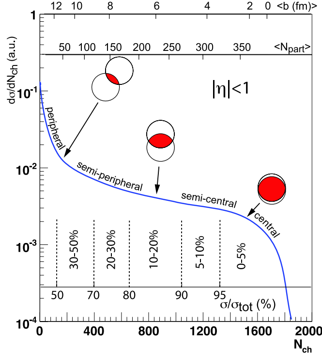
Figure 4.9: An illustrated example of the correlation of the total inclusive charged-particle multiplicity N_{ch} with Glauber-calculated quantities ( b , N_{part} ). The plotted distribution and various values are illustrative and not actual measurements. The figure is taken from [104].
