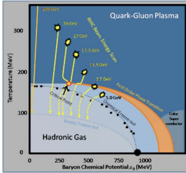
Figure 1.3: A schematic of the phase diagram of nuclear matter. The location of the CP is placed within the RHIC BES range. Lattice QCD estimates indicate that the CP falls within the interval 250 < \mu_B < 450 MeV. The black closed circles are current heavy-ion experimental calculations of the chemical freeze-out temperature, T_{ch} , and \mu_B based on statistical model fits to the measured particle ratios. The yellow curves show the estimated trajectories of the possible collision energies at RHIC. Figure is from [19].
