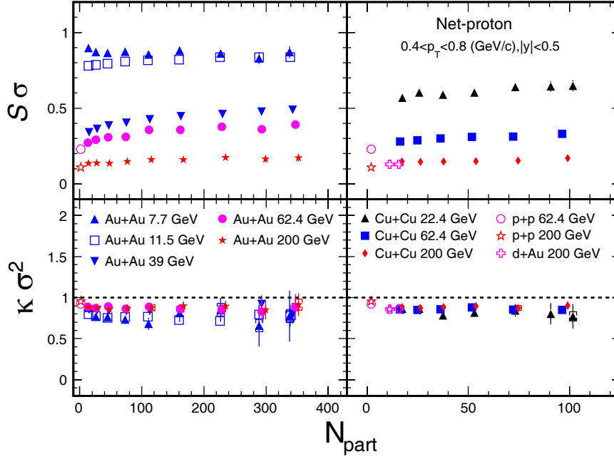
Figure 5.5: Moment products ( \kappa\sigma^2 and S\sigma ) of net-proton distributions for Au+Au, Cu+Cu, d+Au and p+p collisions.
