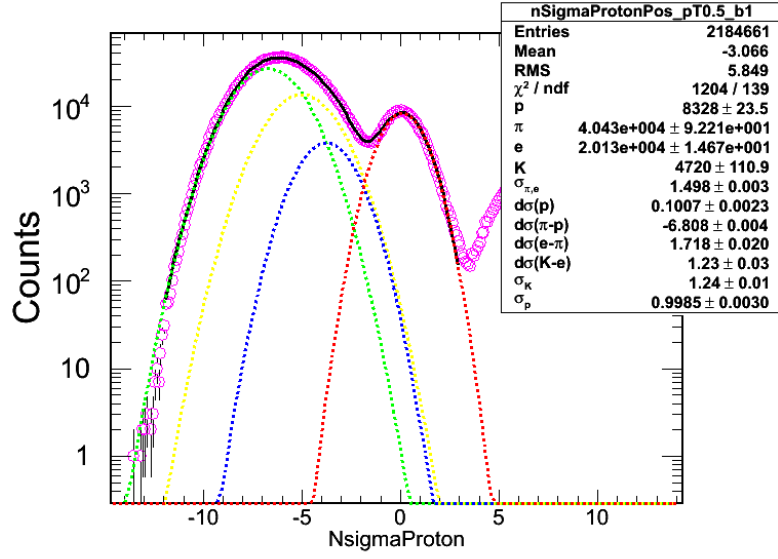
Figure 4.16: NsigmaProton ( Z ) distribution within 0.4 < p_T < 0.5 GeV/ c for Au+Au central collisions at \sqrt{s_{NN}}=7.7 GeV.
