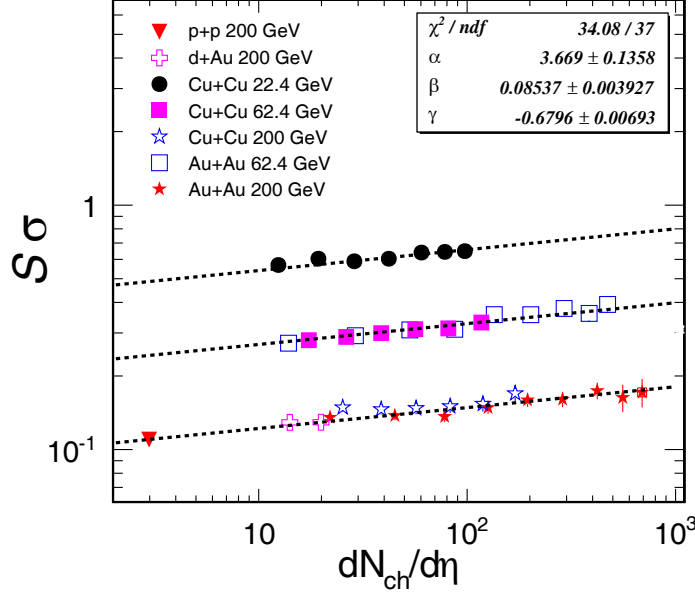
Figure 5.11: S\sigma of net-proton distributions as a function of charged particle density at mid-rapidity ( dN_{ch}/d\eta ) for various colliding systems. The dashed lines in the figures is the fitting lines.
