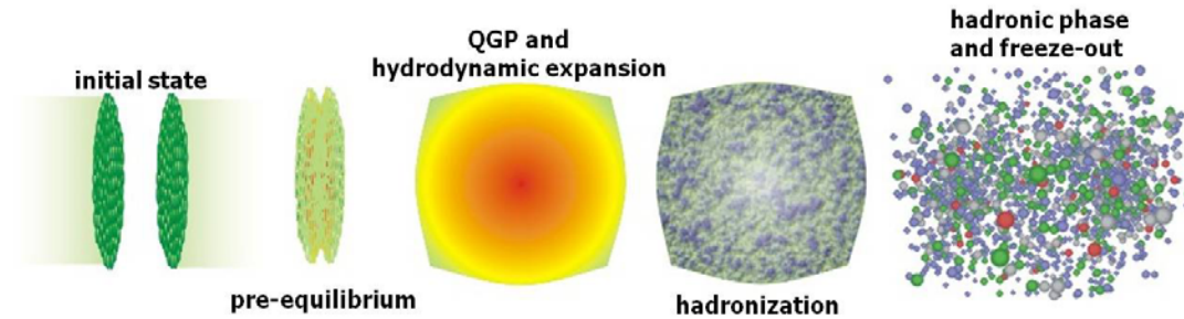
Figure 1.9: Cartoon of a relativistic heavy-ion collision. Left to right: the two nuclei approach, collide, form a QGP, then the QGP expands and hadronization, finally hadrons rescattering and freeze out.
