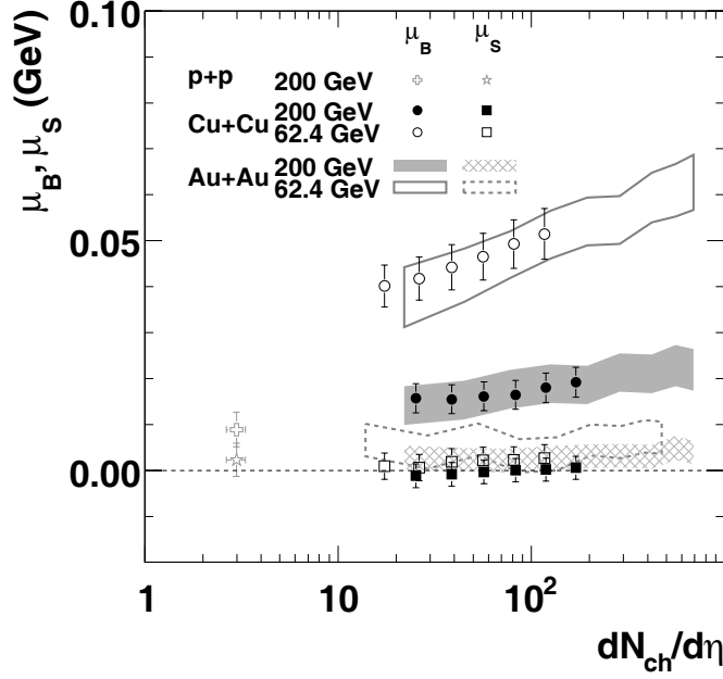
Figure 5.10: Scaling Properties of Chemical Potential: \mu_B and \mu_S versus dN_{ch}/d\eta
