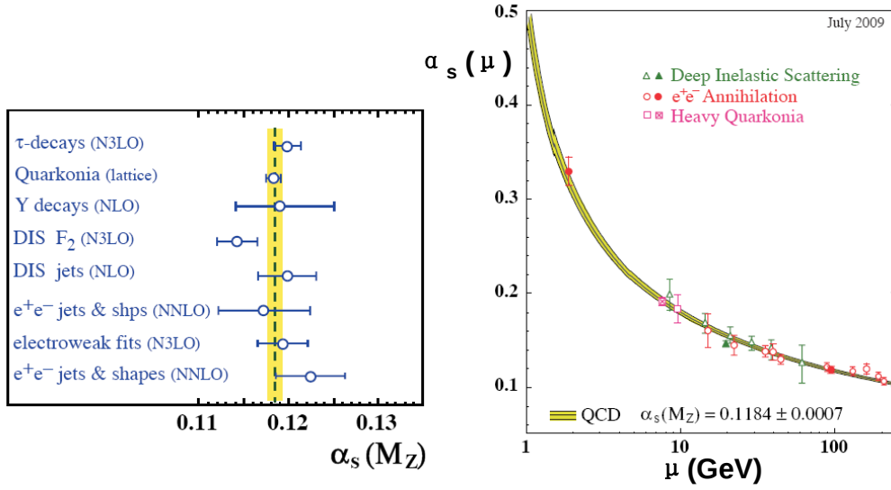
Figure 1.1: Left: Summary of measurements of \alpha_s(M_Z) from different experiments; Right: \alpha_s as a function of the energy scale \mu obtained from Lattice QCD calculations (shadow lines) and experiments (markers). The figures are taken from [7].
