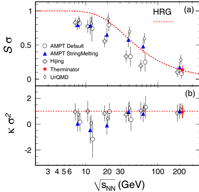
Figure 3.10: Energy dependence of S\sigma and \kappa\sigma^2 of net-proton distributions for various models. The red dash lines are predictions from HRG model.
