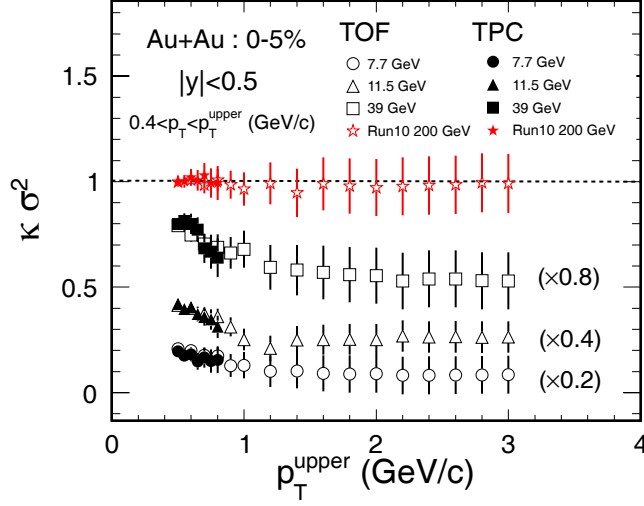
Figure 5.20: \kappa\sigma^2 of net-proton distributions with TPC and TOF PID as a function of p_T coverage for Run 10 Au+Au central collisions at \sqrt{s_{\text{NN}}} = 7.7, 11.5, 39 and 200 GeV.
