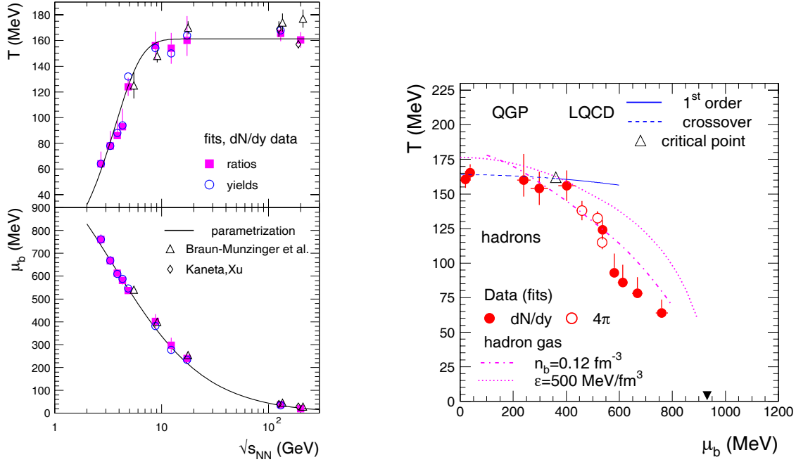
Figure 1.12: Left Panel: The energy dependence of temperature and baryon chemical potential. Right Panel: The experimental values for the chemical freeze-out are shown together with results of lattice QCD calculations. The predicated critical point is marked by open triangle. The freeze-out curve for hadron resonance gas at constant energy density ( \epsilon = 500 MeV/fm 3 ) and constant total baryon density ( n_b = 0.12 fm -3 ) are also included. The full triangle is the ground state of nuclear matter. The figures are taken from [44].
