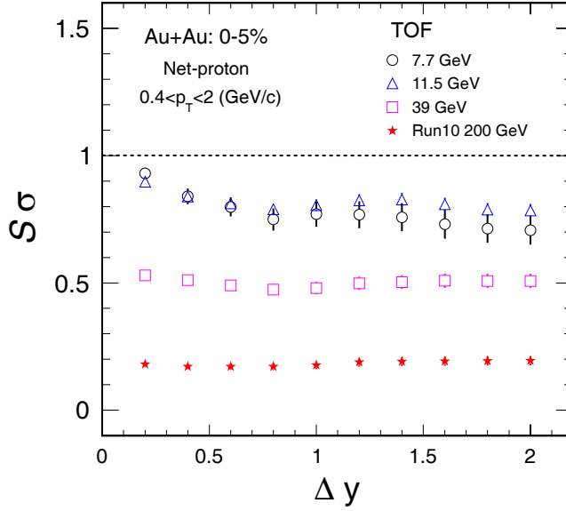
Figure 5.29: Rapidity window size dependence of S\sigma of net-proton distributions with TOF PID for Au+Au central collisions (0 – 5%) at \sqrt{s_{NN}} = 7.7, 11.5, 39 and Run10 200 GeV.
