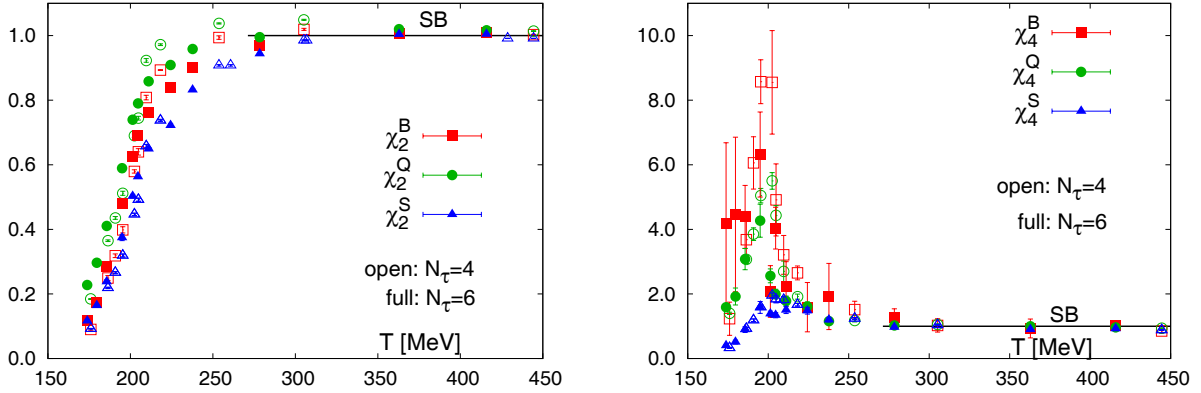
Figure 3.3: Quadratic and quartic fluctuations of net-baryon, net-strangeness and net-charge number at \mu_B = 0 . The figures are taken from [91].
