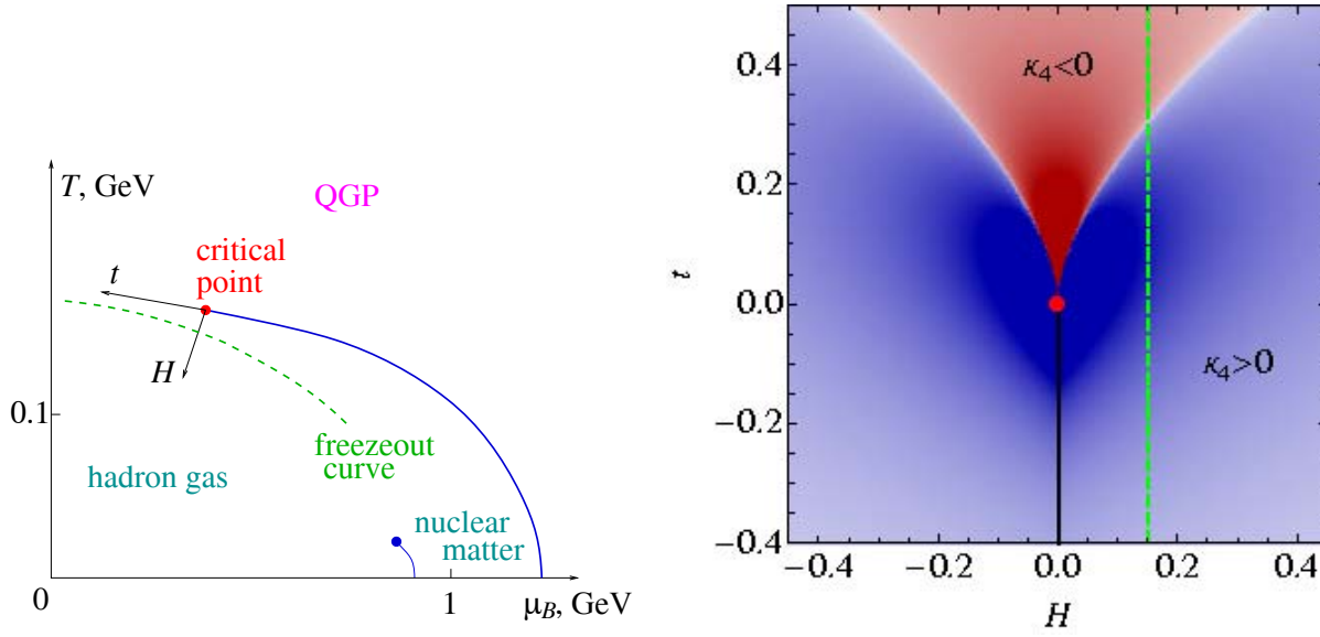
Figure 5.7: Left panel : A sketch of the phase diagram of QCD with the freezeout curve and a possible mapping of the Ising coordinates t and H . Right panel : The density plot of the function \kappa_4(t, H) from the linear parametric model, the \kappa_4 < 0 region is red, the \kappa_4 > 0 is blue. \kappa_4 is the fourth order cumulant. The green dashed lines in left panel and right panel denote the freeze out lines. The figures are taken from [109].
