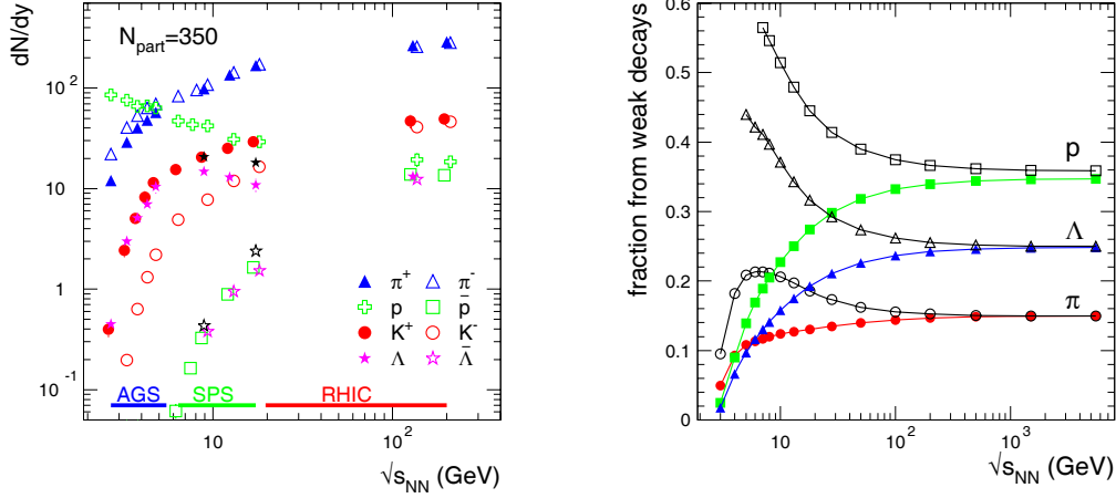
Figure 1.10: Left Panel: The energy dependence of experimental hadron yields at mid-rapidity for various species produced in central heavy ion collisions.
