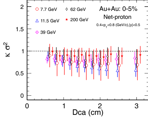
Figure 4.20: \kappa\sigma^2 of net-proton distributions as a function of Dca for Au+Au central collisions (0 – 5%) at \sqrt{s_{NN}} = 7.7, 11.5, 39, 62.4 and 200 GeV.
