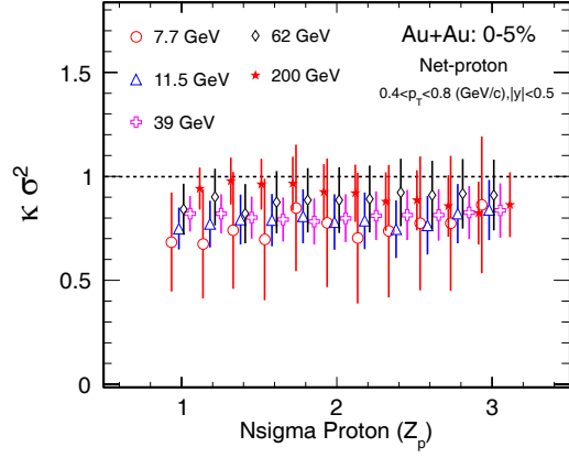
Figure 4.24: \kappa\sigma^2 of net-proton distributions as a function of Nsigma proton ( Z_p ) for Au+Au central collisions (0 – 5%) at \sqrt{s_{NN}} = 7.7, 11.5, 39, 62.4 and 200 GeV.
