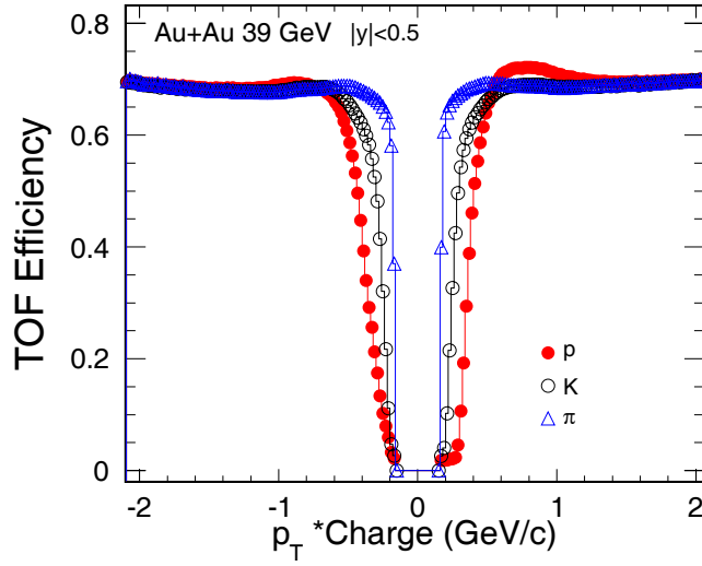
Figure 5.17: TOF matching efficiency for proton, kaon and pion in Au+Au 39 GeV.
