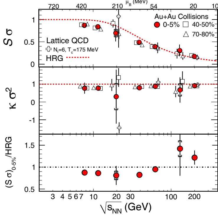
Figure 5.8: Energy dependence of moment products ( \kappa\sigma^2 and S\sigma ) of net-proton distributions for Au+Au collisions central (0 – 5%, 19.6 GeV: 0 – 10%, 130 GeV: 0 – 6%) to peripheral (70 – 80%, 19.6 GeV: 70 – 100%, 130 GeV: 58 – 85%) collisions. The mid-central for 19.6 GeV is 30 – 50%.
