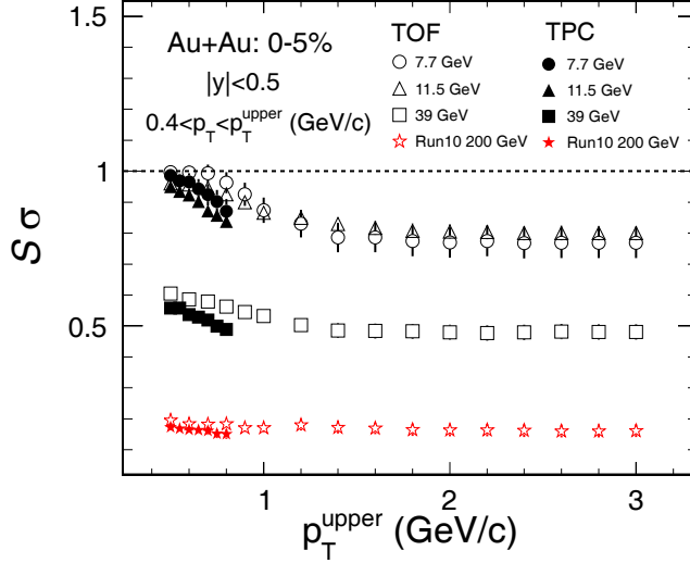
Figure 5.19: S\sigma of net-proton distributions with TPC and TOF PID as a function of p_T coverage for Run 10 Au+Au central collisions at \sqrt{s_{NN}} = 7.7, 11.5, 39 and 200 GeV.
