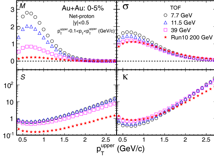
Figure 5.21: Various Moments ( M, \sigma, S, \kappa ) of net-proton distributions as a function of differential p_T coverage with TOF PID for Au+Au central collisions at \sqrt{s_{NN}} = 7.7, 11.5, 39, 200 GeV
