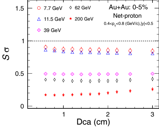
Figure 4.19: S\sigma of net-proton distributions as a function of Dca for Au+Au central collisions (0 – 5%) at \sqrt{s_{NN}} = 7.7, 11.5, 39, 62.4 and 200 GeV.
