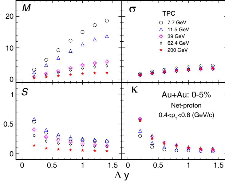
Figure 5.24: Various Moments ( M, \sigma, S, \kappa ) of net-proton distributions as a function of rapidity window size with TPC PID for Au+Au central collisions at \sqrt{s_{NN}} = 7.7, 11.5, 39, 62.4, 200 GeV.
