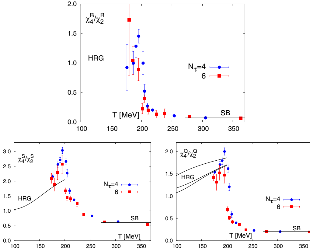
Figure 3.7: The ratio of fourth and second order cumulants of baryon number (top), strangeness (bottom left) and electric charge (bottom right) fluctuations. In the latter case the curves are for a HRG model calculated with physical pion masses (upper curve), pions of mass 220 MeV (middle) and infinitely heavy pions (lower curve). The figures are taken from [57].
