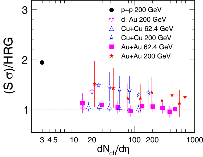
Figure 5.13: S\sigma of net-proton distributions over HRG calculations ratio as a function of charged particle density at mid-rapidity ( dN_{ch}/d\eta ) for various colliding systems within 0.4 < p_T < 0.8 GeV/ c and |y| < 0.5 .
