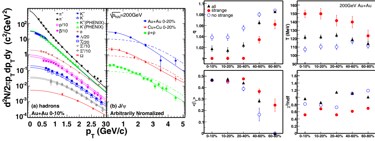
Figure 1.13: Left Side : Identified particle spectra from Au+Au collisions at \sqrt{s_{NN}}=200 GeV. The left panel: spectra of light hadrons and strange hadrons. The solid curves are results from TBW fit. the right panel: J/\psi spectrum, the dashed line is the TBW prediction using parameters from the fit to other hadrons, and the solid curve is a TBW fit to J/\psi alone. Right Side : q , T , \beta and \chi^2/\text{nDoF} as a function of centrality for different groups of hadrons from the TBW model fit to spectra in Au+Au collisions at \sqrt{s_{NN}}=200 GeV. The figures are taken from [47].
