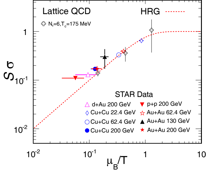
Figure 5.12: S\sigma of net-proton distributions as a function of baryon chemical potential over temperature ratio ( \mu_B/T ) for various colliding systems. The red dashed line in the figures is the result of the HRG model. Lattice QCD results with N_\tau = 6 and T_c = 175 MeV are also shown in the figure.
