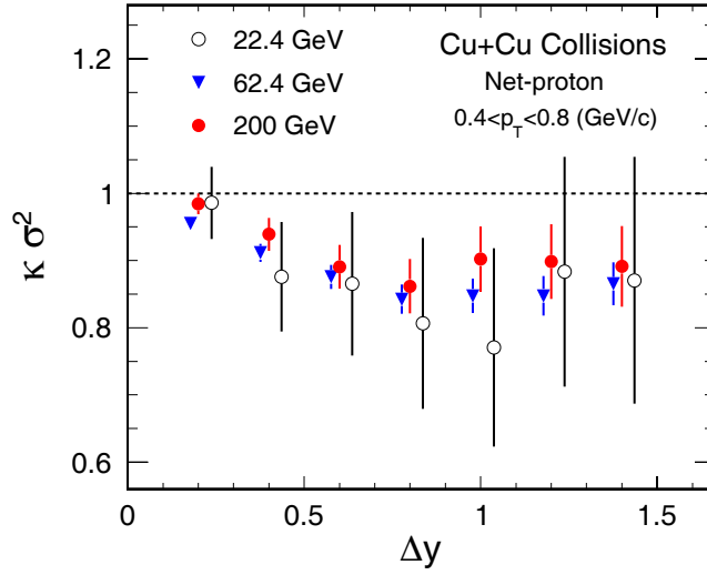
Figure 5.28: Rapidity window size dependence of \kappa\sigma^2 for Cu+Cu central collisions (0 – 10%, 22.4 GeV: 0 – 5%) at \sqrt{s_{NN}} = 22.4, 62.4, 200 GeV.
