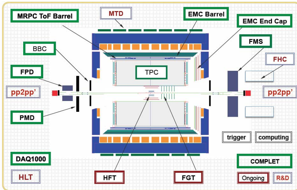
Figure 2.4: Cutaway side view of the STAR detector in year 2008 run and future upgrades.
