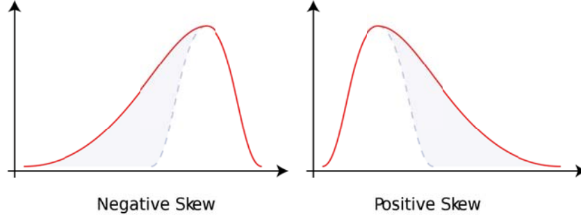
Figure 3.1: Visual example of distribution with negative skewness (left panel) and positive skewness (right panel). The figure is taken from [89].
