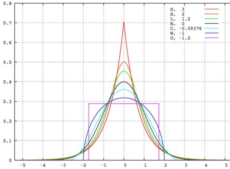
Figure 3.2: Visual example of kurtosis for seven well-known distributions from different parametric family. The figure is taken from [90].
