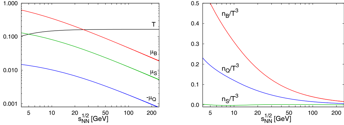
Figure 3.4: The energy dependence of the baryon, strangeness and charge chemical potential at the chemical freeze-out (left part) and the corresponding number density in the right part of the figure. The figures are taken from [58].
