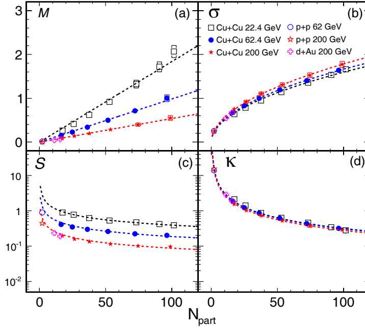
Figure 5.4: Centrality dependence of various moments of net-proton multiplicity distributions for Cu+Cu collisions at \sqrt{s_{NN}} = 22.4, 62.4 and 200 GeV, d+Au collisions at \sqrt{s_{NN}} = 200 GeV and p+p collisions at \sqrt{s_{NN}} = 62.4 and 200 GeV. The dash lines shown in the figure are expectation lines from Central Limit Theorem (CLT).
