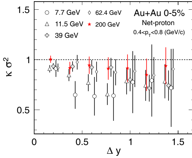
Figure 5.26: Rapidity window size dependence of \kappa\sigma^2 for Au+Au central collisions (0 – 5%) at \sqrt{s_{\text{NN}}} = 7.7, 11.5, 39, 62.4 and 200 GeV.
