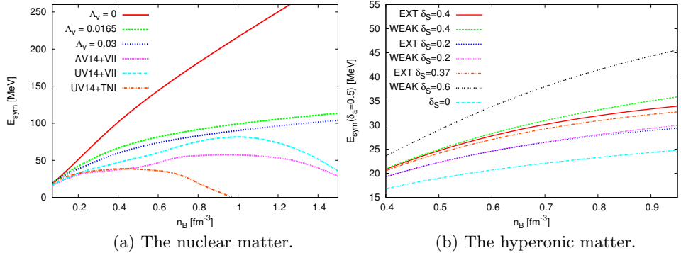
Fig. 2. Left panel: The density dependence of symmetry energy calculated for different values of parameter \Lambda_V and compared with the results obtained for the realistic nuclear potential models [14]. Right panel: The density dependence of symmetry energy calculated for chosen value of parameter \Lambda_V = 0.0165 in the case of asymmetric strangeness-rich matter ( \delta_a = 0.5 ); \delta_S = 0.37 and \delta_S = 0.6 represent the maximal values of strangeness fraction achievable in the maximum mass configuration for extended and weak model, respectively.
