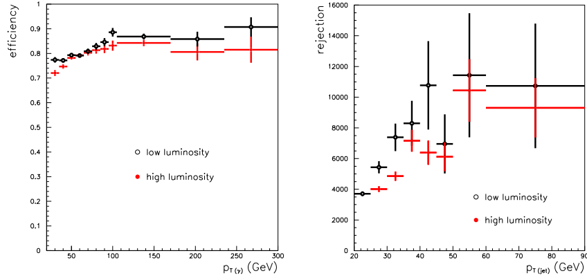
Fig. 1. Efficiency (left) and jet rejection (right) as a function of p_T at low and high luminosity including track isolation cut.
