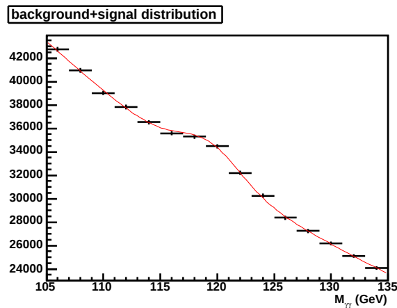
Fig. 3. Expected H \rightarrow \gamma\gamma signal for a M_H = 120 GeV Higgs boson for 100 \text{ fb}^{-1} of integrated luminosity.
