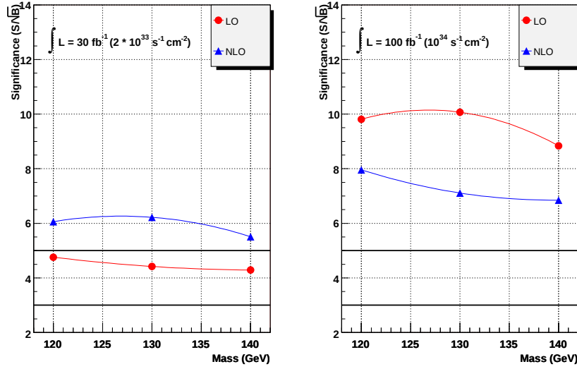
Fig. 4. Statistical significance as a function of the Higgs mass for 30 \text{ fb}^{-1} of integrated luminosity collected in low luminosity conditions ( 2 \times 10^{33} \text{ cm}^{-2} \text{ s}^{-1} ) and 100 \text{ fb}^{-1} of integrated luminosity collected in high luminosity conditions ( 10^{34} \text{ cm}^{-2} \text{ s}^{-1} ) using both LO and NLO cross sections.
