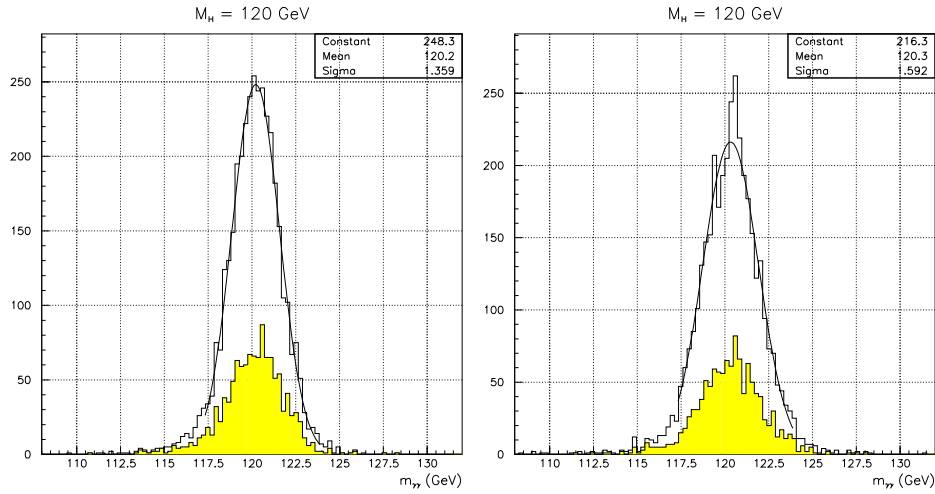
Fig. 2. Reconstructed two photons invariant mass for H \rightarrow \gamma\gamma decay at low (left) and high luminosity (right). The lower histograms represent events containing at least one converted photon.
