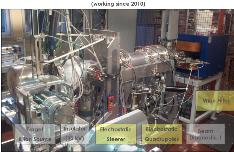
Fig. 4. The SPES test bench: from the left-hand side one can observe the proton beam line, the TIS system, the insulator, the electrostatic steerer, the electrostatic quadrupole and, finally, the Wien Filter selector.
