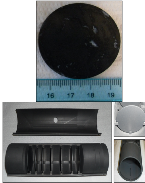
Fig. 3. The SPES multi-foil \text{UC}_x target.
