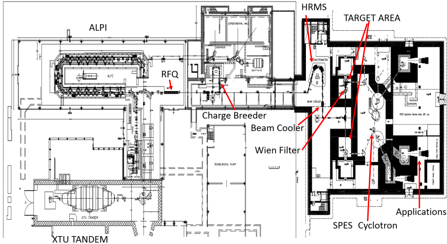
Fig. 1. The SPES layout.
