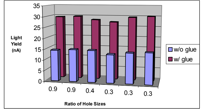
Fig. 3. Average Light Yield With and Without Glue.
