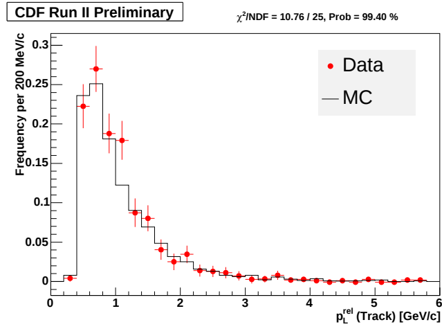
Figure 4.25: p_L^{\text{rel}} spectrum of tracks in a cone \Delta R = 0.7 around the B_s meson; data (red) and Monte Carlo (black).
