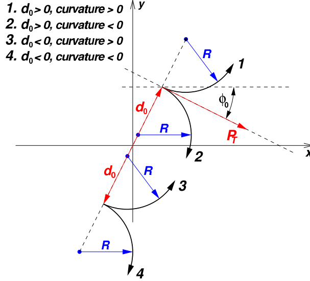
Figure 3.4: Illustration of helix track parametrization.
