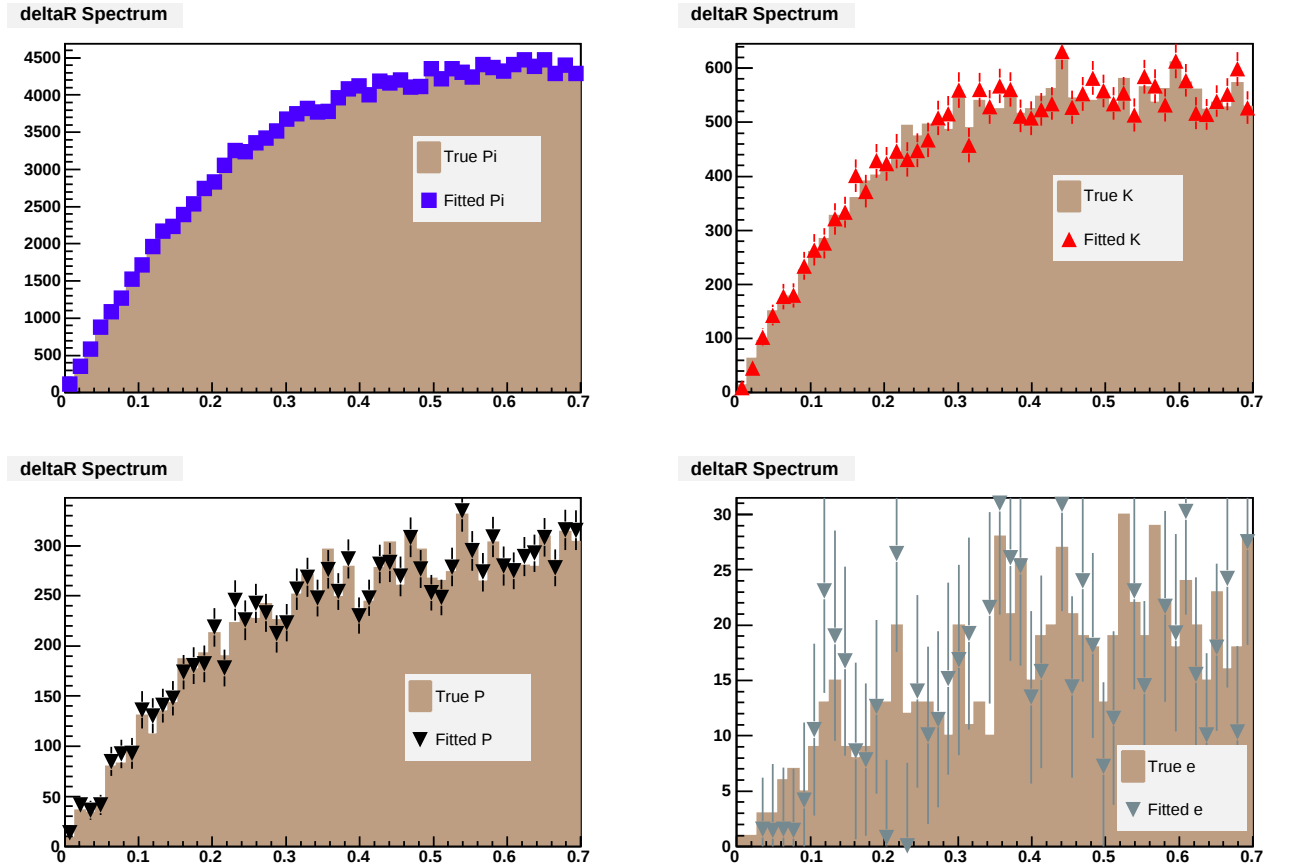
Figure 6.15: Pythia MC \Delta R = \sqrt{\Delta\eta^2 + \Delta\phi^2} distributions overlaid to the corresponding data sPlot of each particle species.
