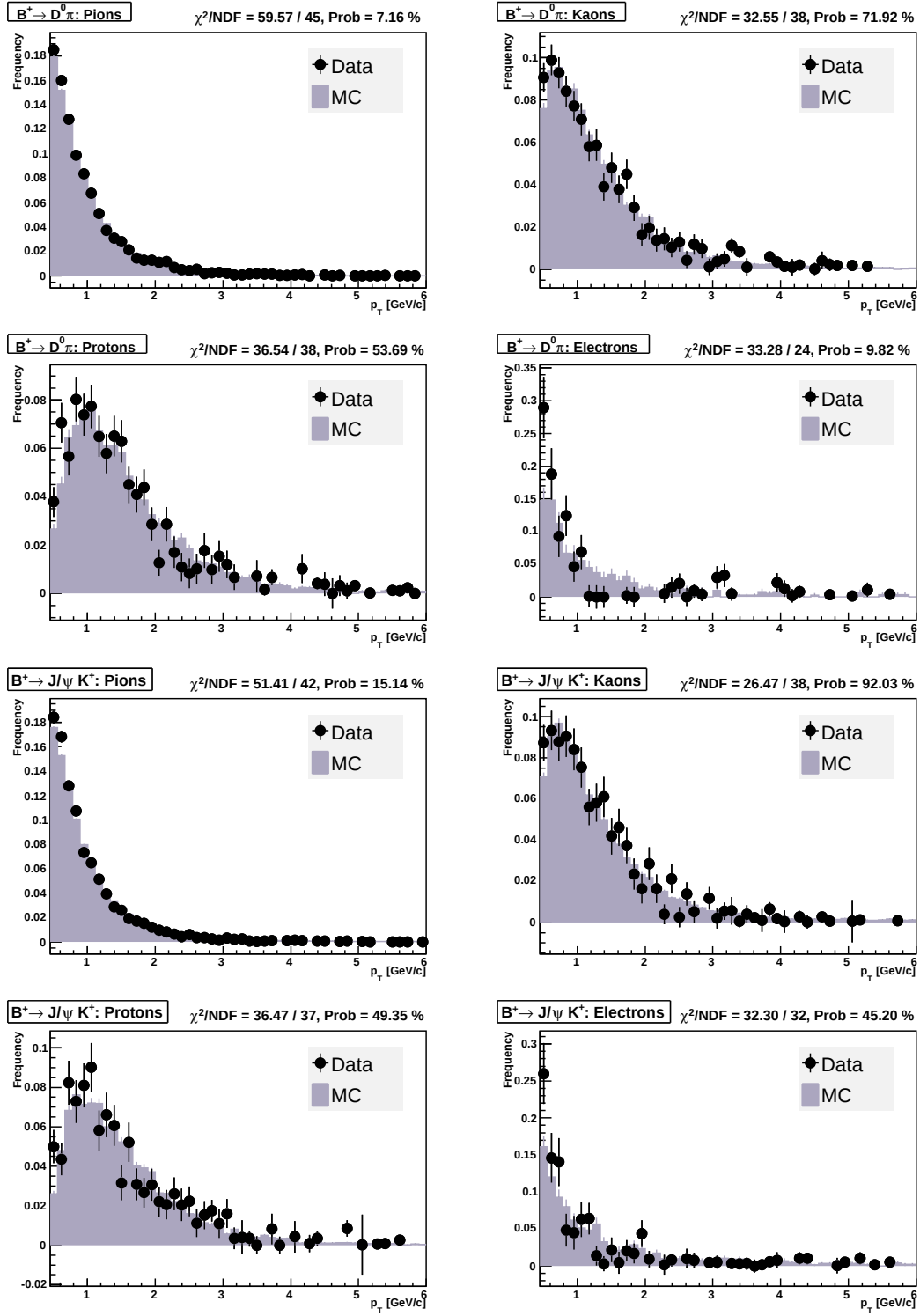
Figure 8.3: B^+ \rightarrow \overline{D}^0 \pi^+ and B^+ \rightarrow J/\psi K^+ , P_T distributions of particle species seen around the B meson direction.
