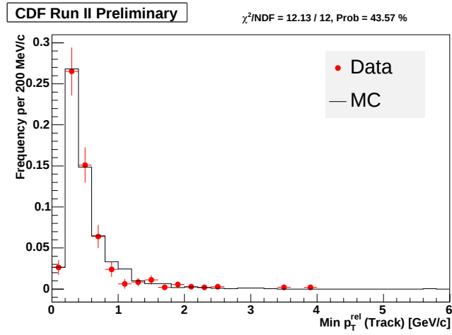
Figure 4.26: \text{Min } p_T^{\text{rel}} spectrum of tracks in a cone \Delta R = 0.7 around the B_s meson; data (red) and Monte Carlo (black).
