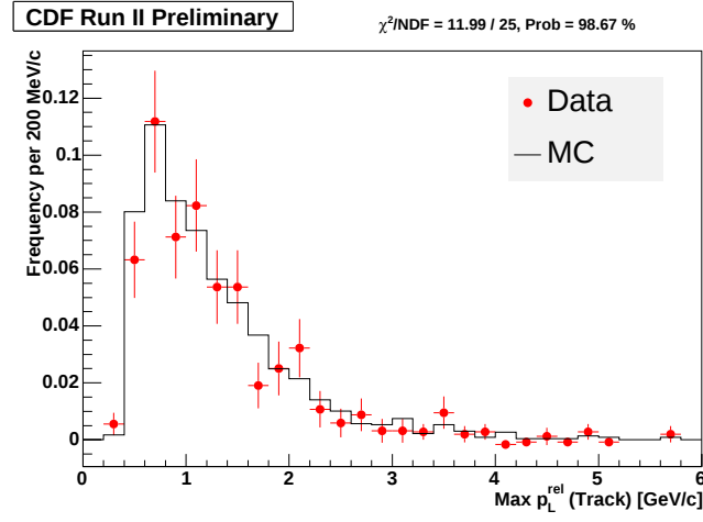
Figure 4.27: \text{Max } p_L^{\text{rel}} spectrum of tracks in a cone \Delta R = 0.7 around the B_s meson; data (red) and Monte Carlo (black).
