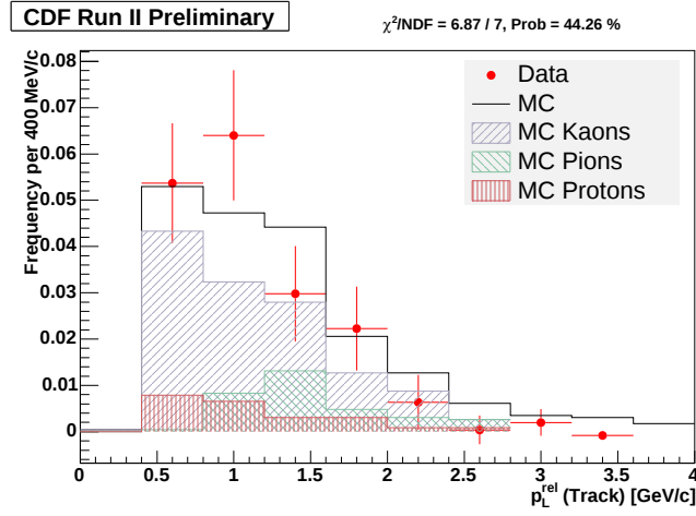
Figure 4.34: p_L^{\text{rel}} spectrum of tracks passing LR_{\text{comb}} > -1 cut in a cone \Delta R = 0.7 around the B_s meson; data (red) and Monte Carlo (black).
