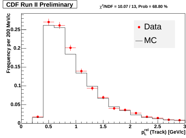
Figure 4.7: p_L^{rel} spectrum of tracks in a cone \Delta R = 0.7 around the B_u meson; data (red) and Monte Carlo (black).
