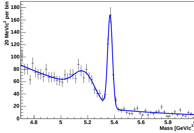
Figure 4.2: Invariant mass distribution for B_s events.
