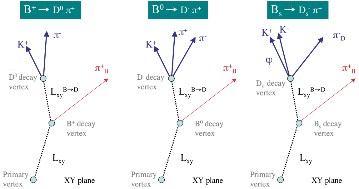
Figure 5.2: Picture of the hadronic decay modes considered.
