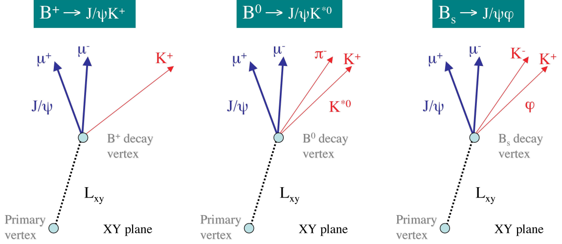
Figure 5.1: Picture of the J/\psi decay modes considered.
