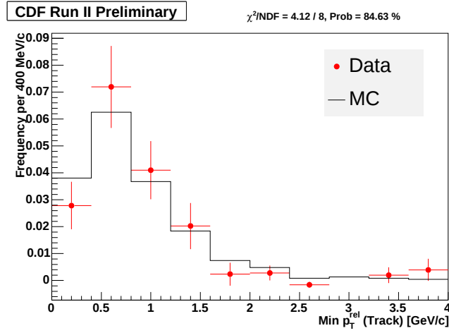
Figure 4.35: \text{Min } p_T^{\text{rel}} spectrum of tracks passing LR_{\text{comb}} > -1 cut in a cone \Delta R = 0.7 around the B_s meson; data (red) and Monte Carlo (black).
