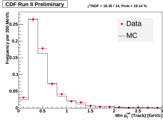
Figure 4.8: \text{Min } p_T^{rel} spectrum of tracks in a cone \Delta R = 0.7 around the B_u meson; data (red) and Monte Carlo (black).
