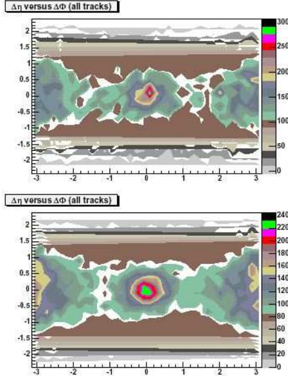
Figure 5.11: The track activity in the \Delta\phi - \Delta\eta plane around the B meson in data (top) and Pythia Monte Carlo (bottom) for B^+ \rightarrow J/\psi K^+ events. The activity of the other b -hadron is also visible.
