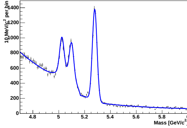
Figure 4.1: Invariant mass distribution for B_u events.
