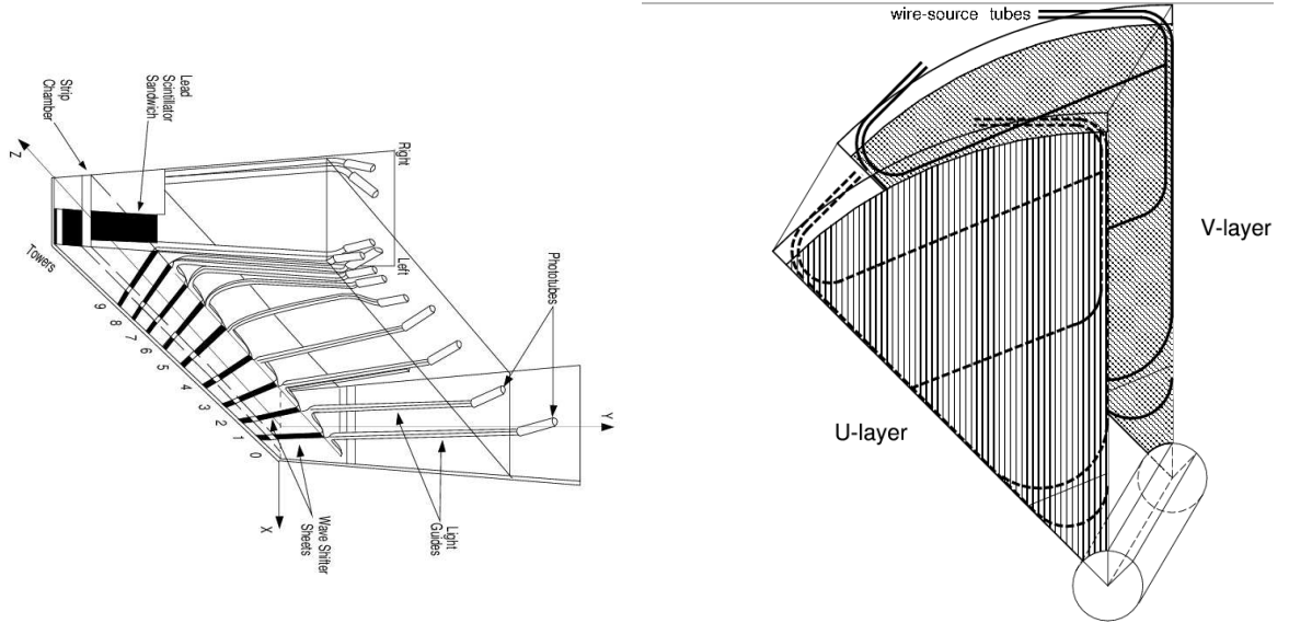
Figure 3.14: Perspective view of a CEM module (left) and of SMD (right).
