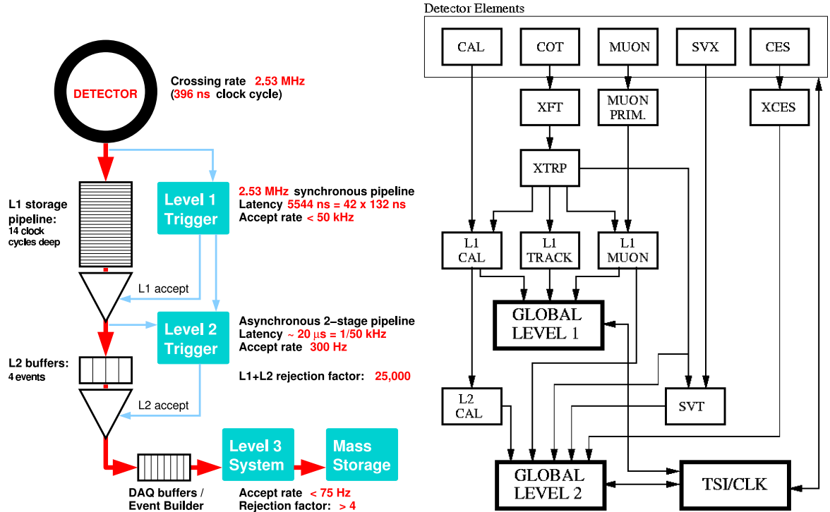
Figure 3.16: Block diagram detailing CDF DAQ and L1/L2 trigger system.
