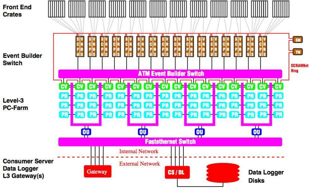
Figure 3.20: Event Builder and L3 operating principle. All the main components are shown: ATM switch (purple), converter nodes (green), output nodes (dark blue), Consumer Sever and data logging System (red).
