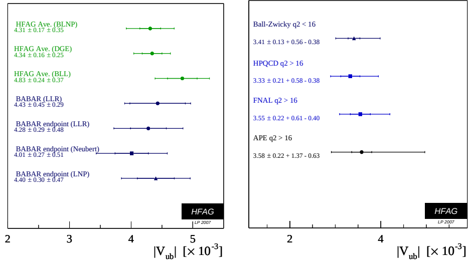
Fig. 2. Calculations of |V_{ub}| from inclusive b \rightarrow u \ell \nu decays (left) and exclusive B \rightarrow \pi \ell \nu as performed by the Heavy Flavor Averaging Group [14]. The theoretical frameworks for the inclusive determinations are described in references [12, 15–19]. The references for the form factor calculations are described in [20–23]. The inner error bars show the experimental uncertainty, while the full error bars show the experimental and theoretical uncertainties added in quadrature.
