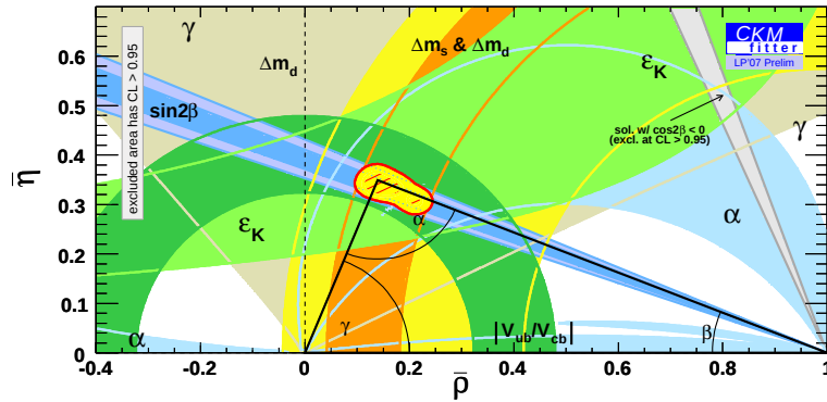
Fig. 1. Constraints on the apex of the Unitarity Triangle (\bar{\rho}, \bar{\eta}) as of the Lepton-Photon '07 conference from the CKMfitter group [7].
