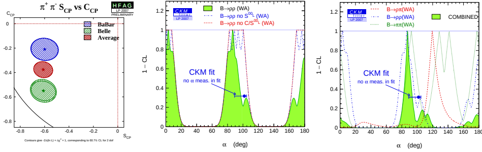
Fig. 3. The plot on the left shows the latest measurements of the time-dependent CP violation coefficients S and C for B^0 \rightarrow \pi^+\pi^- . Figure courtesy of the heavy flavor averaging group [14]. The middle and right plots show constraints on the Unitarity Triangle angle \alpha from the isospin analysis of the \rho\rho system (middle) and from \pi\pi , \rho\rho , and \rho\pi combined. Figures courtesy of the CKMfitter group [7].
