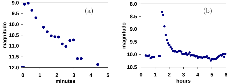
Fig. 2. (a) — Outburst of CN Leo flare star automatically detected 2005.04.02 1:13:42 UT = 3462.55620 HJD. (b) — Outburst of EQ Peg flare star 2004.09.19. Time in hours after 2453267.56 HJD. Peak at 2453267.6224.
