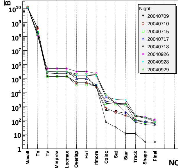
Fig. 1. Number of events \bar{B} at specific stages of the triggering system, normalised for a single camera for 10-hours long night.
