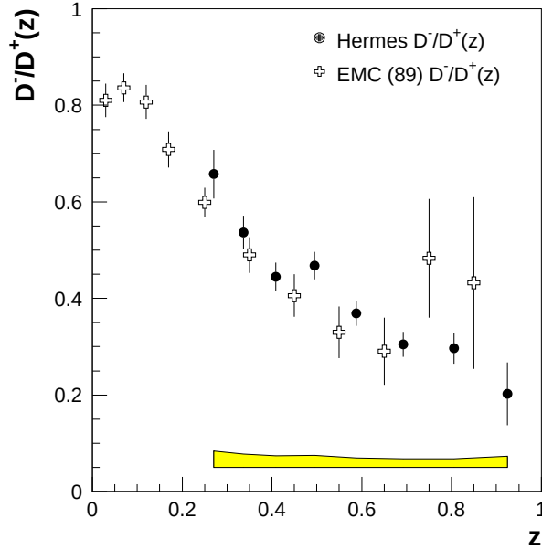
Fig. 8. Comparison of preliminary data on the ratio D^-(z)/D^+(z) as measured with HERMES to the results of EMC [12]. The error band shows the systematic error of the HERMES measurement.
