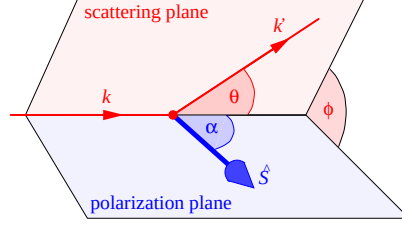
Fig. 2. Definition of scattering angles in polarised deep inelastic scattering. The four vectors of the incident and scattered lepton are denoted by k = (E, \vec{k}) and k' = (E', \vec{k}') . The lepton scattering angle is called \theta . \hat{S} gives the target polarisation direction and \phi is the angle between the polarisation plane (defined by \vec{k} and \hat{S} ) and the scattering plane (defined by \vec{k} and \vec{k}' ). \alpha is the angle between the beam momentum \vec{k} and the target polarisation \hat{S} .
