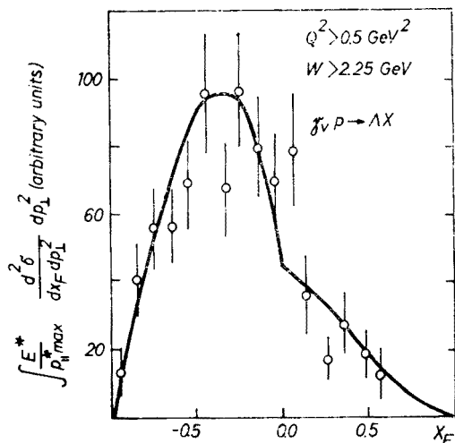
Fig. 4. Feynman x_F = 2p_{\parallel h}^*/W distribution of electroproduced \Lambda from the Cornell-DESY collaboration [21] compared with the typical baryon spectrum from quark and diquark jet fragmentation
