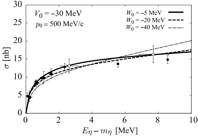
Fig. 3. Calculated escape part \sigma_{\text{esc}} in Fig. 2 is plotted with the experimental data of the d + d \rightarrow \eta + \alpha reaction indicated by black squares [8], black circles [9], and open circles [10]. The parameters of the \eta - \alpha optical potential are (V_0, W_0) = -(30, 5) , -(30, 20) , and -(30, 40) MeV and the p_0 parameter is fixed to be p_0 = 500 MeV/ c . The line is roughly fitted to data by eye.
