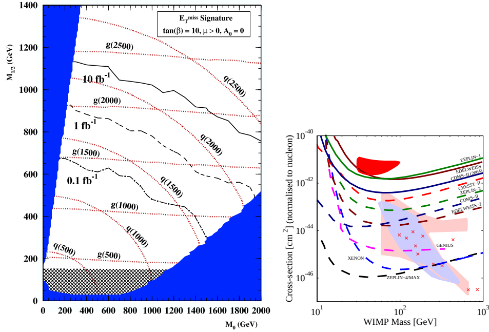
Fig. 5. Left: Contours in a parameter space of supersymmetry models for the discovery of the missing energy plus jets signature of new physics by the ATLAS experiment at the LHC. The three sets of contours correspond to levels of integrated luminosity at the LHC (in \text{fb}^{-1} ), contours of constant squark mass, and contours of constant gluino mass [8]. Right: Sensitivities of some running and planned direct detection dark matter experiments to the spin-independent elastic scattering cross-section. Full curves correspond to limits from existing experiments, dashed curves to predicted sensitivities of future experiments. The full dark region corresponds to the 3\sigma allowed region from the DAMA experiment. The full light regions correspond to predictions in the light of WMAP data. The crosses correspond to neutralino masses and cross-sections predicted for post-LEP benchmark CMSSM models [9].
