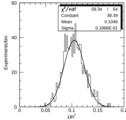
Fig. 6. Distribution of the predicted relic density \Omega_\chi h_0^2 for the SPA benchmark model incorporating the experimental errors (the uncertainty on the position of the \tau\tau edge is assumed to be 5 GeV) [11].
