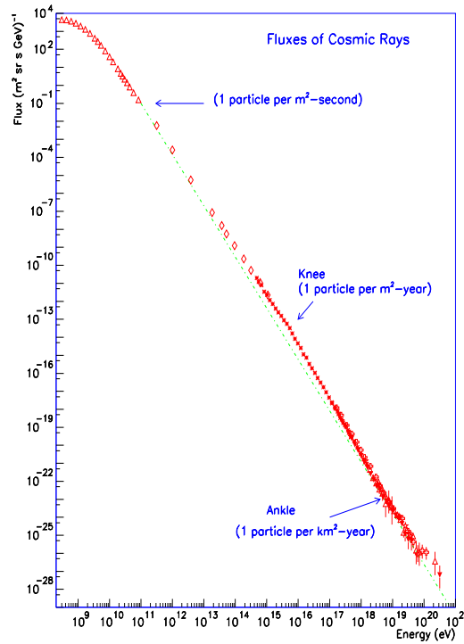
Fig. 1. Global energy spectrum of cosmic rays giving the differential flux in terms of energy.
