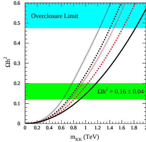
Fig. 4. Prediction for \Omega_{B^{(1)}} h_0^2 . The solid line is the case for B^{(1)} alone, and the dashed and dotted lines correspond to the case in which there are one (three) flavors of nearly degenerate e_R^{(1)} . There are several curves associated with various values of the mass difference between the e_R^{(1)} and B^{(1)} [7].
