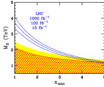
Fig. 7. Comparison of the regions covered by LHC (with respective integrated luminosities 1000, 100 and 10 \text{ fb}^{-1} ) and the Pierre Auger Observatory in 5 years in the plane (M_D, x_{\min}) (see text) [15].
