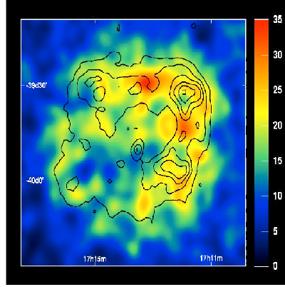
Fig. 2. \gamma -ray image of the supernova remnant RX J1713.7-3946 with the H.E.S.S. telescopes.
