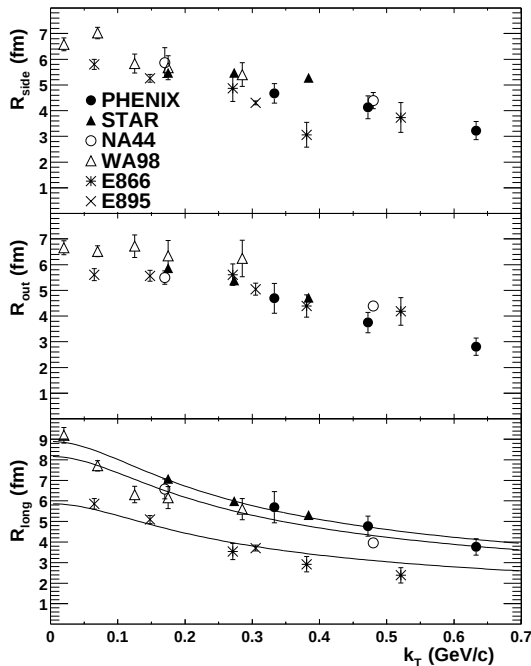
Fig. 1. Summary of HBT radii for pion pairs in heavy-ion collisions as a function of k_T measured at mid-rapidity for various energies from E895 ( \sqrt{s_{NN}} = 4.1 GeV), E866 ( \sqrt{s_{NN}} = 4.9 GeV), NA44, WA98 ( \sqrt{s_{NN}} = 17.3 GeV), STAR, and PHENIX ( \sqrt{s_{NN}} = 130 GeV). The bottom plot includes fits to A/\sqrt{m_T} for each energy region. The data are for \pi^- results except for the NA44 results, which are for \pi^+ . Results are from [7] and references therein.
