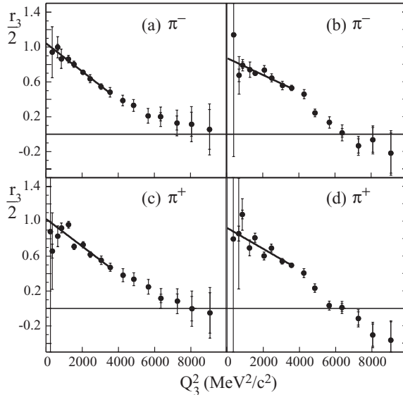
Fig. 2. 130 GeV Au–Au collisions measured by the STAR collaboration in (a) central and (b) mid-central \pi^- events and (c) central and (d) mid-central \pi^+ events.
