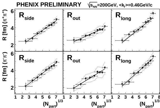
Fig. 3. Scaling of HBT parameters with number of participants ( N_{\text{part}} ).
