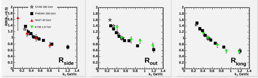
Fig. 4. Comparison of relative k_T dependence of heavy-ion and proton-proton HBT parameters. All radii are normalized to their values at k_T \approx 0.5 .
