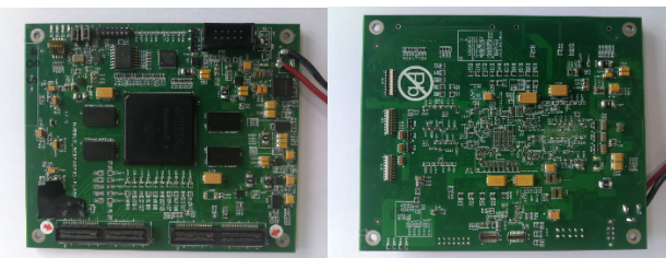
Figure 6: Digital controller motherboard.
