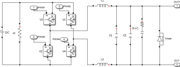
Figure 2: Internal simulation diagram of module.
