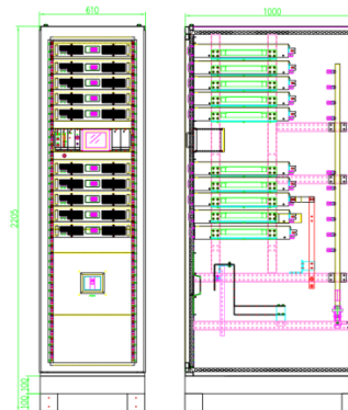
Figure 11: The power cabinet.
