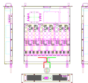
Figure 10: Modular mechanical drawing.
