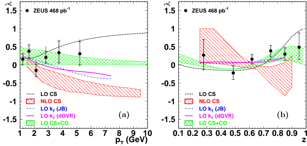
Figure 1: The helicity parameter \lambda , measured in the target frame, as a function of (a) p_T , and (b) z . The measurement is performed in the kinematic range 50 < W < 180 GeV, 0.1 < z < 1 and p_T > 1 GeV. The measurement as a function of p_T is restricted to the kinematic range 0.4 < z < 1 . The inner (outer) error bars correspond to the statistical (total) uncertainty. The theoretical curves are described in the text.
