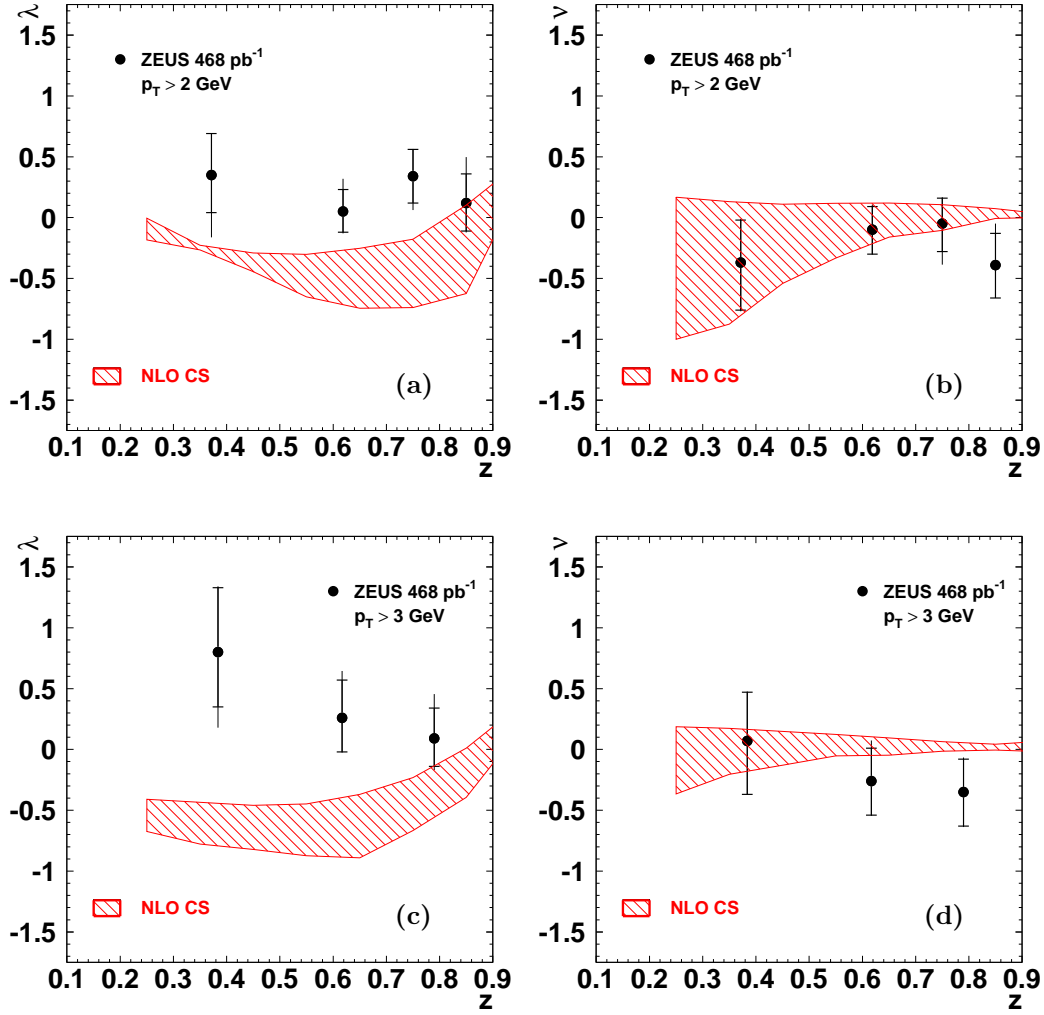
Figure 3: Distributions of the helicity parameters (a), (c) \lambda and (b), (d) \nu as a function of z , measured in the target frame, for 50 < W < 180 GeV, 0.1 < z < 0.9 and (a), (b) p_T > 2 GeV and (c), (d) p_T > 3 GeV. The inner (outer) error bars correspond to the statistical (total) uncertainty. The theoretical bands are described in the text.
