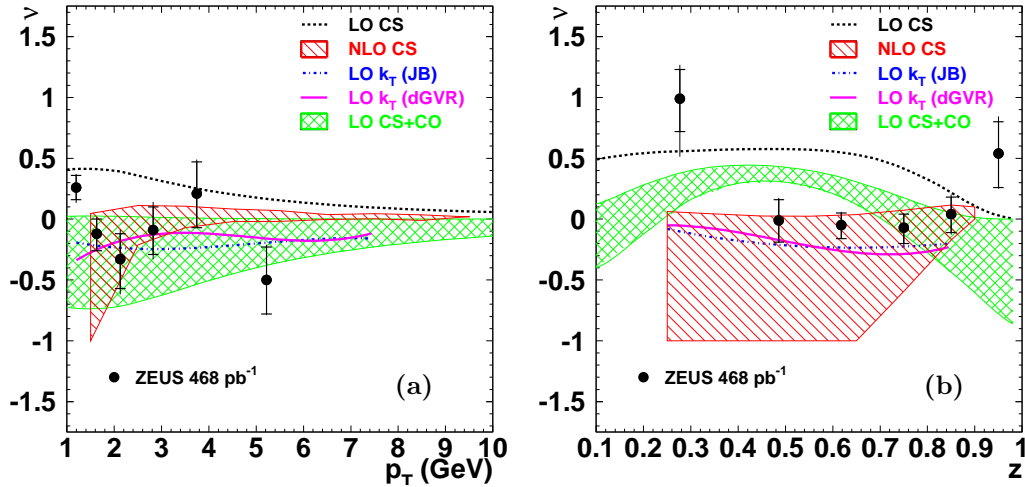
Figure 2: The helicity parameter \nu , measured in the target frame, as a function of (a) p_T , and (b) z . The measurement is performed in the kinematic range 50 < W < 180 GeV, 0.1 < z < 1 and p_T > 1 GeV. The measurement as a function of p_T is restricted to the kinematic range 0.4 < z < 1 . The inner (outer) error bars correspond to the statistical (total) uncertainty. The theoretical curves are described in the text.
