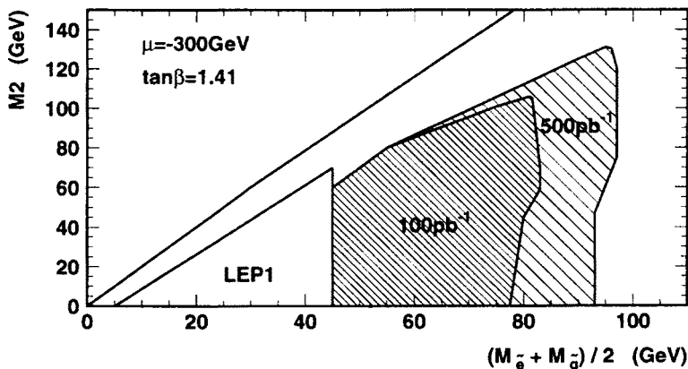
Fig. 1. Exclusion limits for HERA from the process ep \rightarrow \bar{e}qX at 95% C.L. assuming two integrated luminosities 100 \text{ pb}^{-1} and 500 \text{ pb}^{-1} . The small triangle is the region already excluded by LEP1 and the diagonal line is the limit where the lightest neutralino has the same mass as the selectron or squark. Figure taken from Ref. [18].
