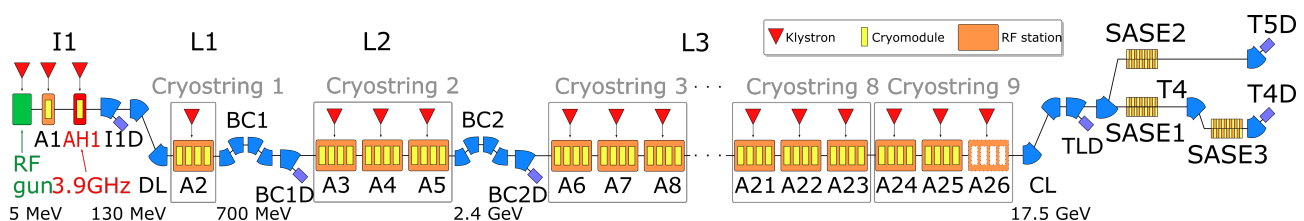
Figure 1: Schematic of the RF stations, the cryostrings and the accelerator sections of the European XFEL.
