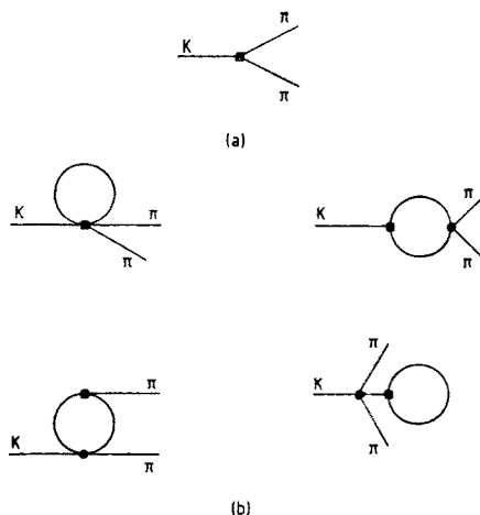
Fig. 19. The (a) leading and (b) next-to-leading contributions to the \Delta S = 1 K \rightarrow \pi\pi decay amplitudes
