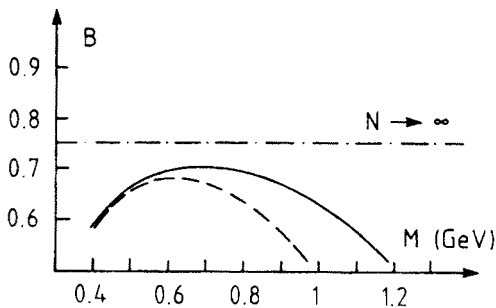
Fig. 25. The B -parameter without (dashed) and with (full) vector meson contributions as a function of the cut-off, for \Lambda_{\text{QCD}} = 0.3 GeV
