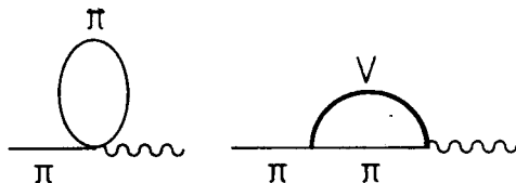
Fig. 29. Pseudoscalar and vector meson next-to-leading corrections to the decay constant f_\pi
