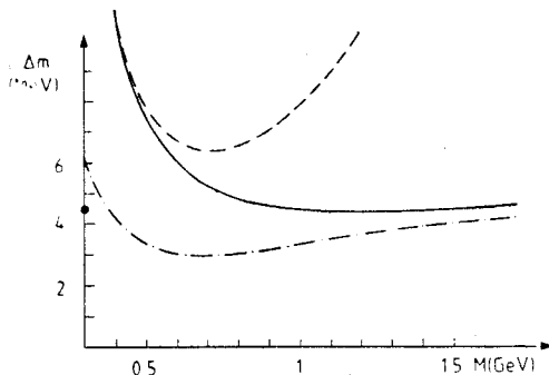
Fig. 16. The \pi^+ - \pi^0 electromagnetic mass difference as a function of the cut-off M (scale where we match the meson and quark-gluon pictures). (a) Dashed line: long-distance part calculated with pseudoscalar mesons only and with \Lambda_{\text{QCD}} = 0.3 GeV, \hat{m}(1 \text{ GeV}) = 4.6 MeV; (b) Full line: long-distance part calculated with pseudoscalar, vector and axialvector mesons and with \Lambda_{\text{QCD}} = 0.3 GeV, \hat{m}(1 \text{ GeV}) = 4.6 MeV; (c) Dashed-dotted line: same as (b) but with \Lambda_{\text{QCD}} = 0.2 GeV and \hat{m}(1 \text{ GeV}) = 6.9 MeV. The experimental value is represented by a black dot
