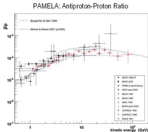
Figure 3: PAMELA: antiproton-proton ratio (preliminary)
