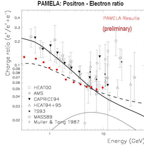
Figure 4: PAMELA: e^+/(e^-+e^+) ratio (preliminary)
