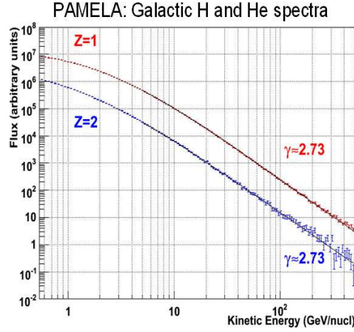
Figure 5: PAMELA: proton and helium energy spectra (preliminary)
