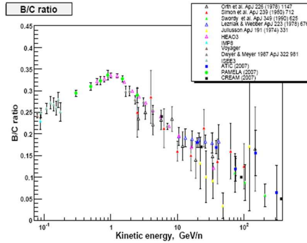
Figure 7: PAMELA: B/C ratio from 300 MeV/n up to 200 GeV/n (preliminary)
