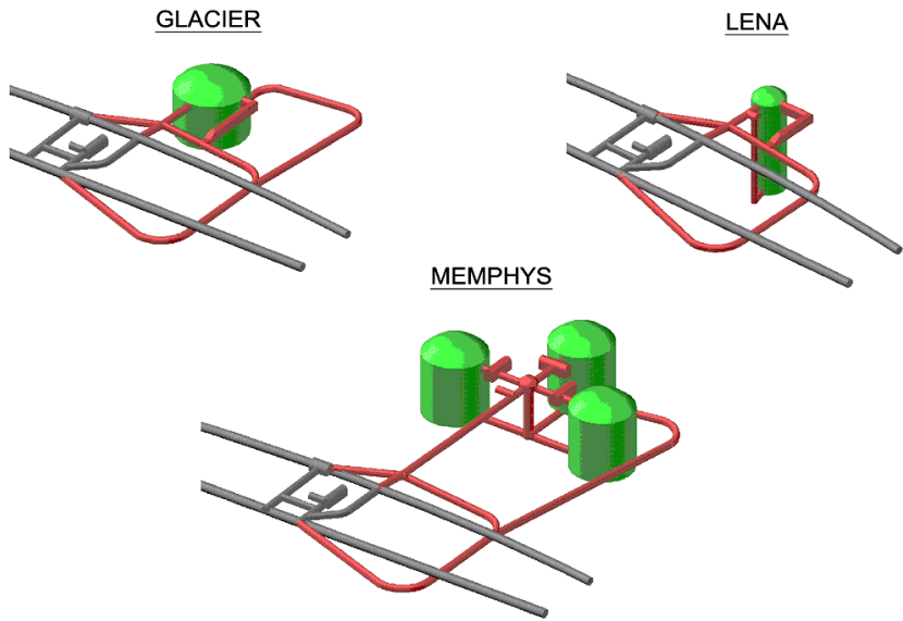
Fig. 2. Possible location near the LSM of each one of the 3 proposed experiments.
