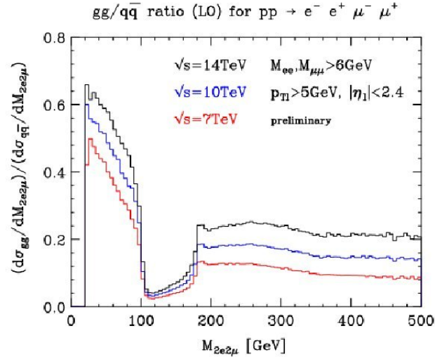
Figure 4.7: gg \rightarrow ZZ contribution relative to q\bar{q} \rightarrow ZZ contribution at different centre-of-mass energies.
