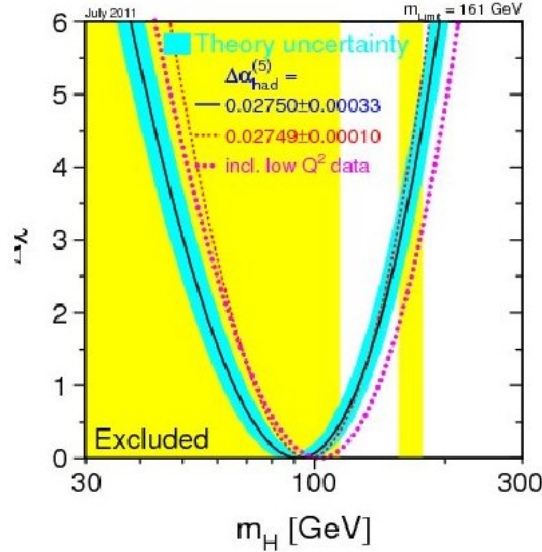
Figure 1.3: \Delta\chi^2 of the fit to the electroweak precision measurements performed at LEP, SLC and Tevatron as a function of the Higgs boson mass (July 2011). The black, solid line represents the result of the fit, and the blue, shaded band is the theoretical error from unknown higher-order corrections. The yellow area represents the regions excluded by LEP-II and Tevatron.
