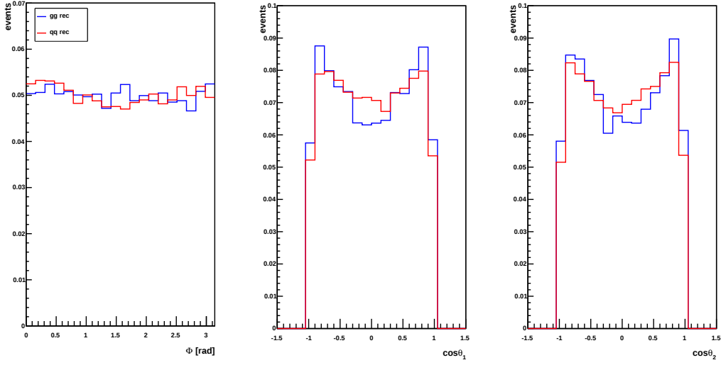
Figure 4.20: \Phi , \cos \theta_1 and \cos \theta_2 distributions at reconstruction level for gg \rightarrow ZZ \rightarrow 2e2\mu and q\bar{q} \rightarrow ZZ \rightarrow 2e2\mu processes at a centre-of-mass energy of 8 TeV.
