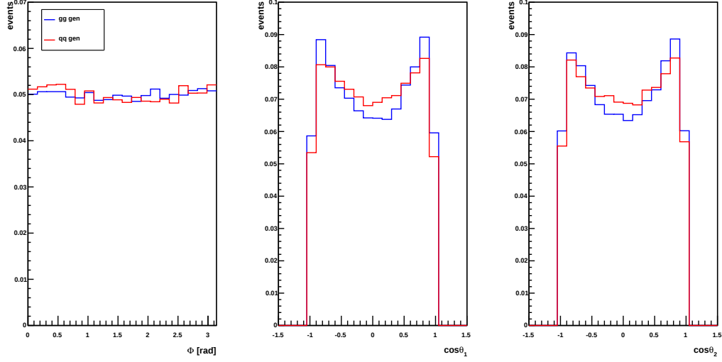
Figure 4.9: \Phi , \cos \theta_1 and \cos \theta_2 distributions at generator level for gg \rightarrow ZZ \rightarrow 2e2\mu and q\bar{q} \rightarrow ZZ \rightarrow 2e2\mu processes at a centre-of-mass energy of 7 TeV.
