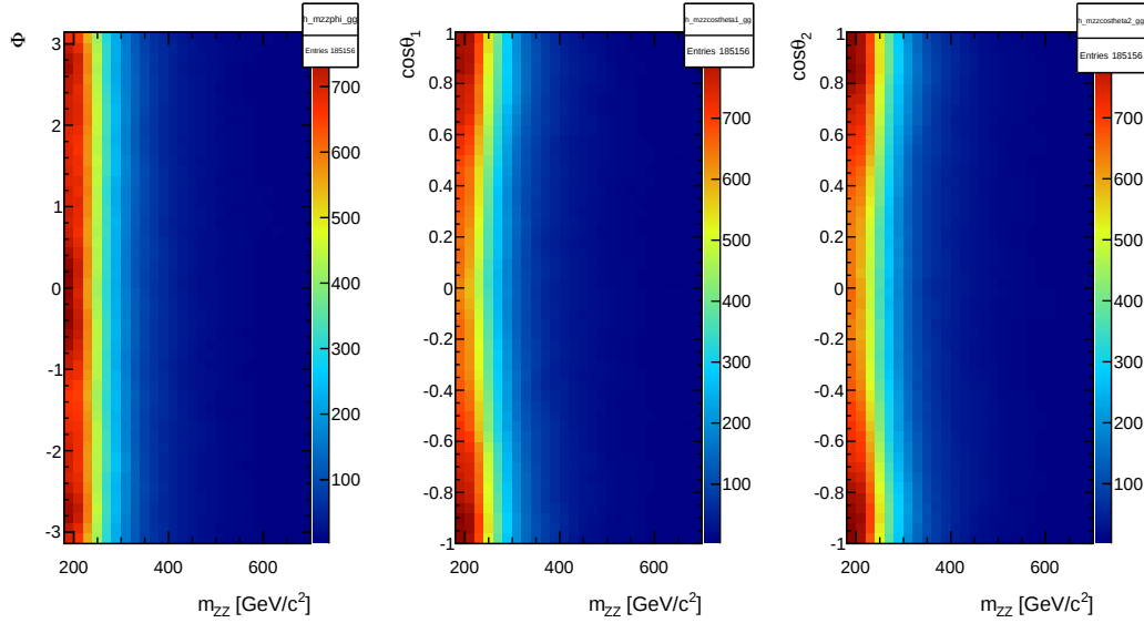
Figure 5.1: \Phi , \cos\theta_1 and \cos\theta_2 distributions as a function of m_{ZZ} at reconstruction level for gg \rightarrow ZZ process at a centre-of-mass energy of 7 TeV. The three channels 2e2\mu , 4e and 4\mu are merged together.
