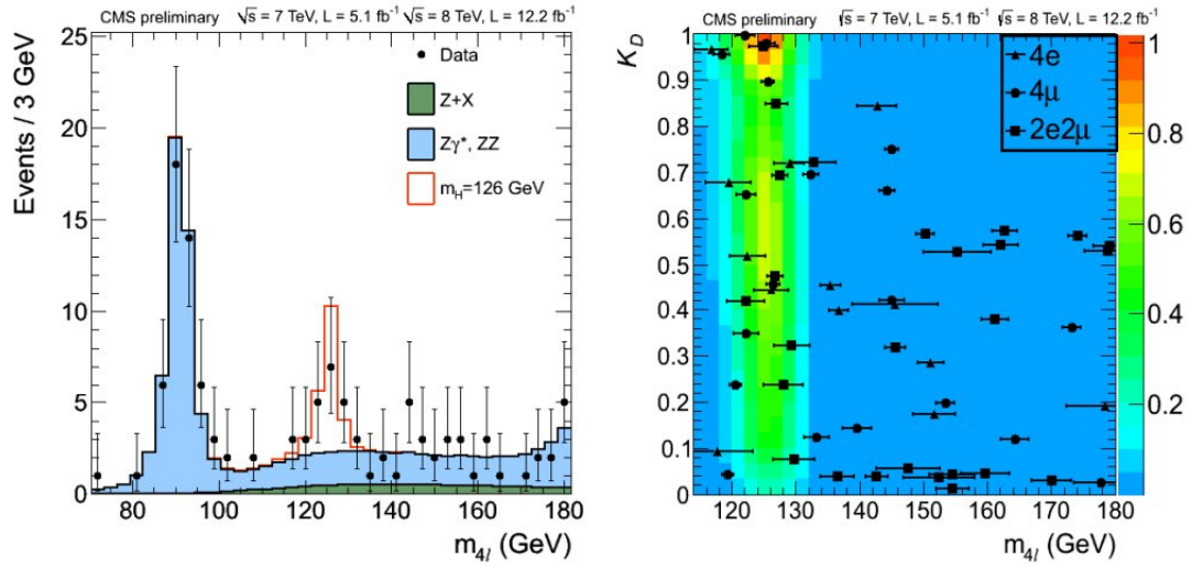
Figure 3.16: Distribution of the four-lepton reconstructed mass for the sum of the 4e, 4μ and 2e2μ channels (left). Points represent the data, shaded histograms represent the background and unshaded histogram the signal expectations. Distribution of the MELA KD versus the four-lepton reconstructed mass m_{4\ell} (right) with contours shown for expected relative density of signal events for hypothesis m_H = 126 GeV/c 2 . The points show data with measured invariant mass uncertainties.
