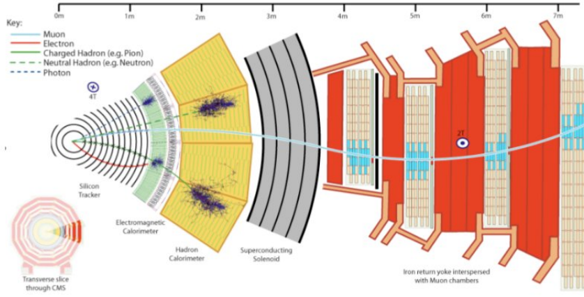
Figure 3.1: Schematic representation of a reconstructed muon track crossing the CMS detector.
