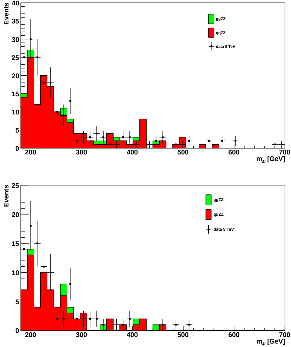
Figure 5.8: Comparison between data and MC for the m_{4\ell} distribution, without (top) and with (bottom) the cut ggMELA > 0.7 , for a centre-of-mass energy of 8 TeV and a luminosity of 12.2 \text{ fb}^{-1} . Points represent data, and histograms represent the gg \rightarrow ZZ and q\bar{q} \rightarrow ZZ background contributions, obtained from MC.
