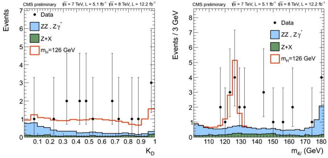
Figure 3.17: Distribution of the MELA kinematic discriminant for events in the mass region 121.5 < m_{4\ell} < 130.5 \text{ GeV}/c^2 (left). Distribution of the four-lepton reconstructed mass for the sum of the 4e , 4\mu and 2e2\mu channels for events with a value K_D > 0.5 of the MELA kinematic discriminant (right). Points represent the data, shaded histograms represent the background and unshaded histogram the signal expectations. The measurements are presented for the sum of the data collected at \sqrt{s} = 7 \text{ TeV} and \sqrt{s} = 8 \text{ TeV} .
