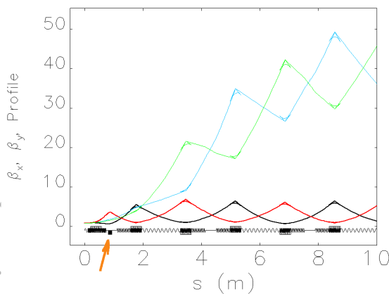
Figure 2: Beta-functions after solenoid in positron linear accelerator. Thick lines (red, black) – structure with additional quadrupole lens (indicated orange), thin lines (green, blue) – plain FODO structure.
