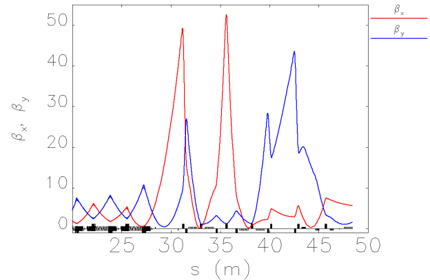
Figure 3: Beta-functions.
