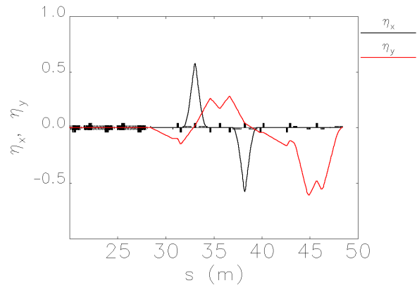
Figure 4: Dispersion functions.
