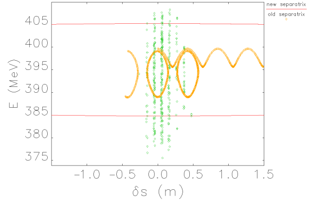
Figure 7: Injected beam in energy separatrix before and after RF-system upgrade.
