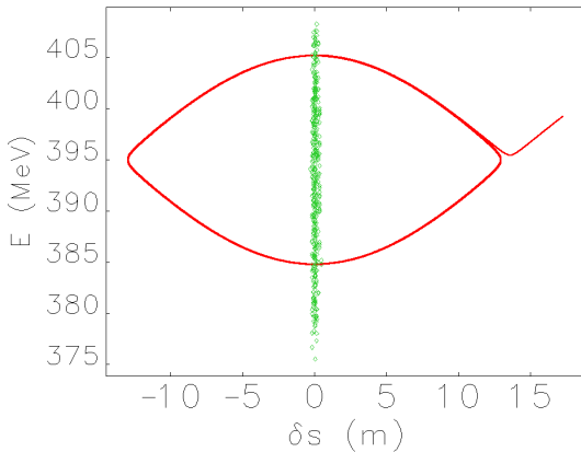
Figure 6: Damping Ring separatrix with injected beam.
