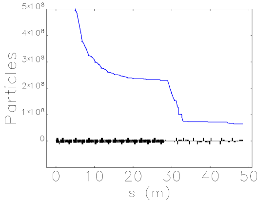
Figure 5: Beam loss in process of positron injection.
