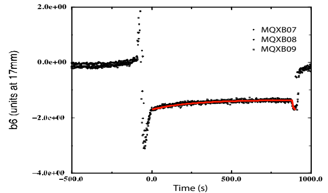
Figure 4: Decay and snapback in the dodecapole field component of the LHC IR quadrupoles.
