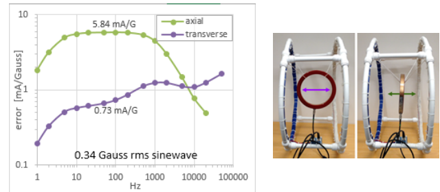
Figure 4: The error from a sinusoidal 1 Gauss external field is 0.7mA for transverse and 5.3mA for axial fields.
