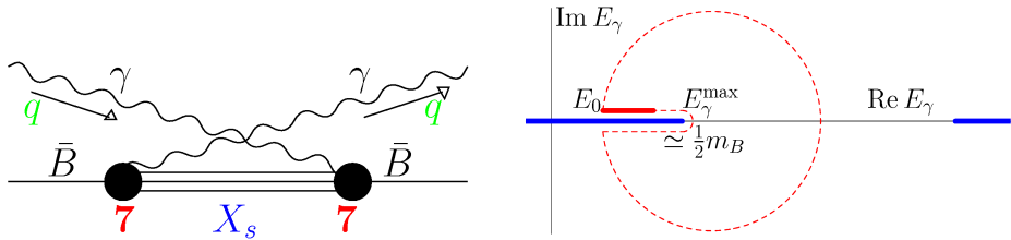
Fig. 2. Left: The amplitude A in Eq. (3). Right: Contour integrals of A (see the text).
