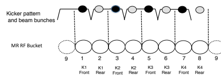
Figure 4: Relationships between beam bunches, kicker fields and rf buckets.
