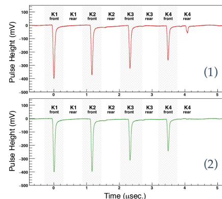
Figure 7: Time structures of beams extracted to the abort beam line.
