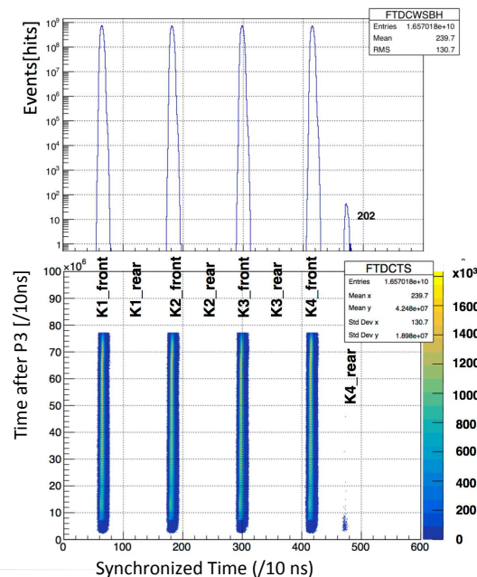
Figure 3: Time spectrum (top) and progress (bottom) of secondary particles.
