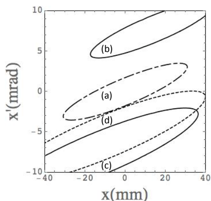
Figure 6: Phase space ellipses at the kicker exit.
