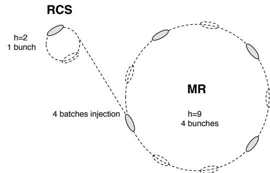
Figure 1: Beam transfer diagram from RCS to MR for COMET.
