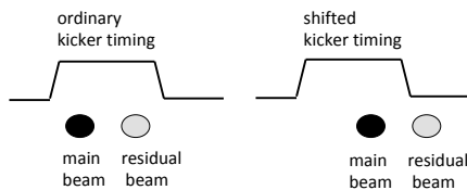
Figure 2: MR injection kicker timing and beam bunches.
