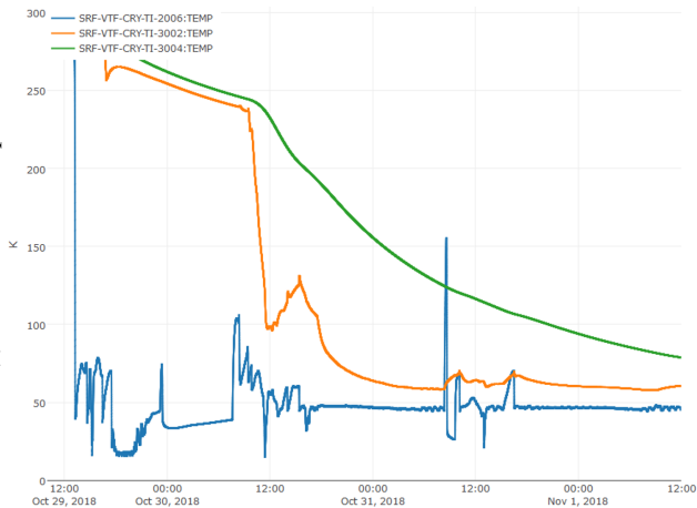
Figure 5: Shield cooldown to 50 K.
