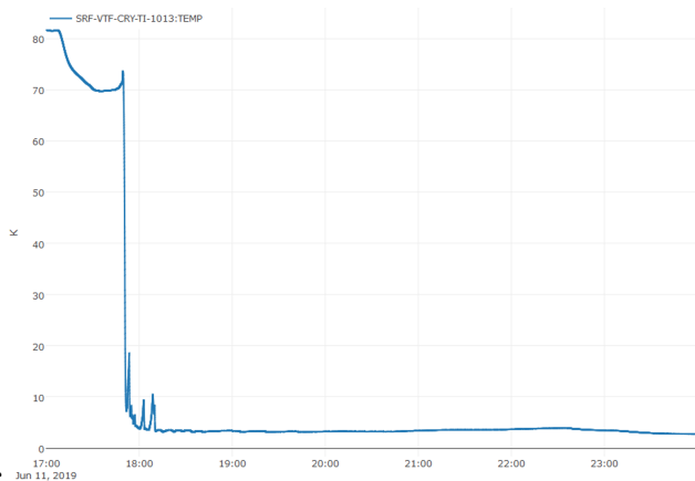
Figure 6: Cavity cooldown to 4 K.
