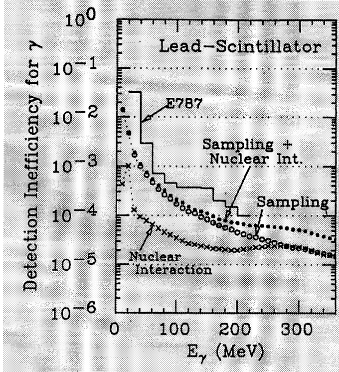
Figure 18: Photon detection inefficiency as a function of energy in lead-scintillator detectors from Ref. [14].
