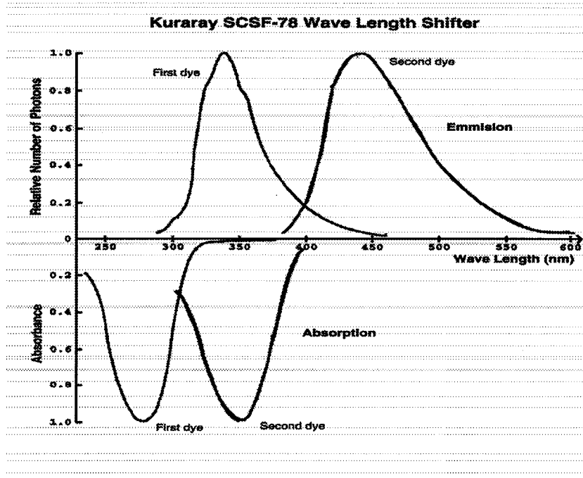
Figure 11: The absorption and emission spectra of the two dyes proposed for the KAMI photon veto detectors. The first dye will be used in the scintillator and the second dye will be used as a wavelength shifter in the fibers.
