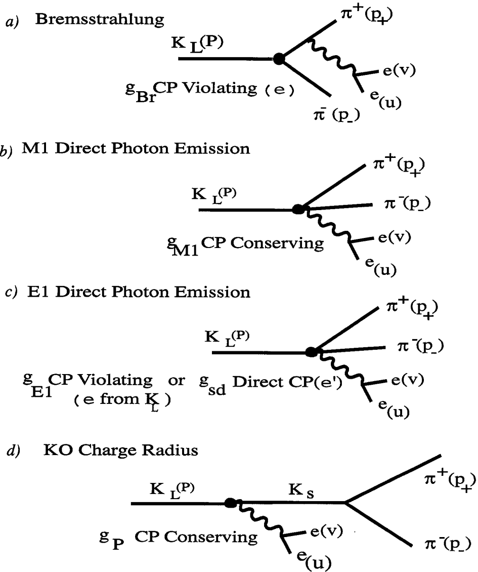
Figure 25: Contributing diagrams to the decay K_L^0 \rightarrow \pi^+\pi^-e^+e^- .
