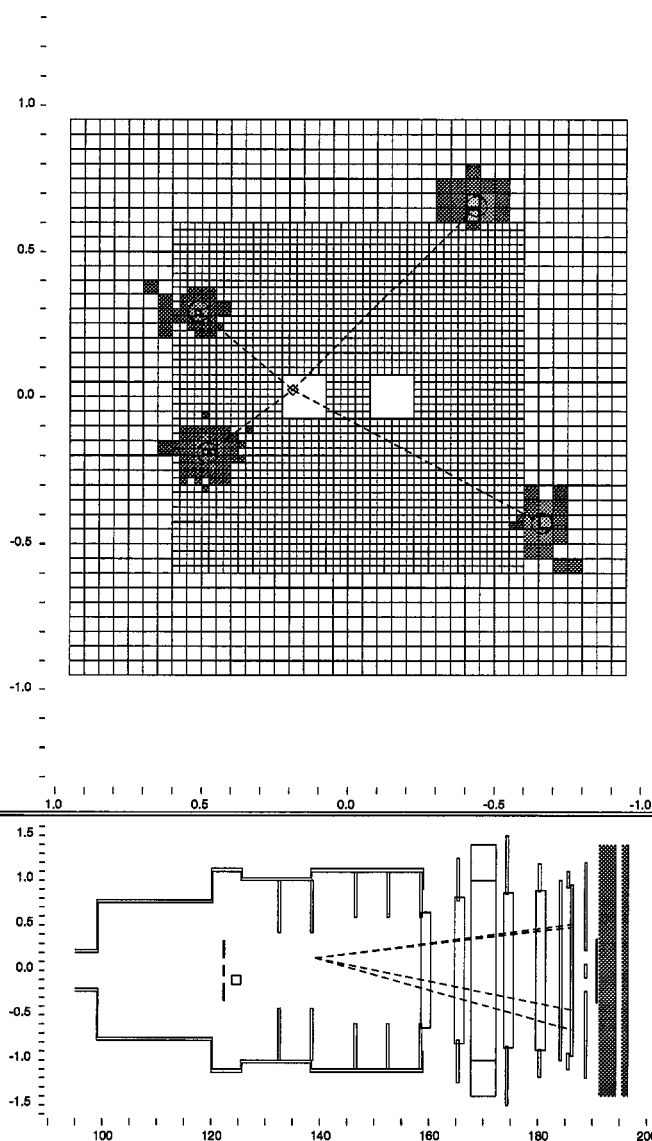
Figure 14: KTeV event display showing a typical 2\pi^0 event.
