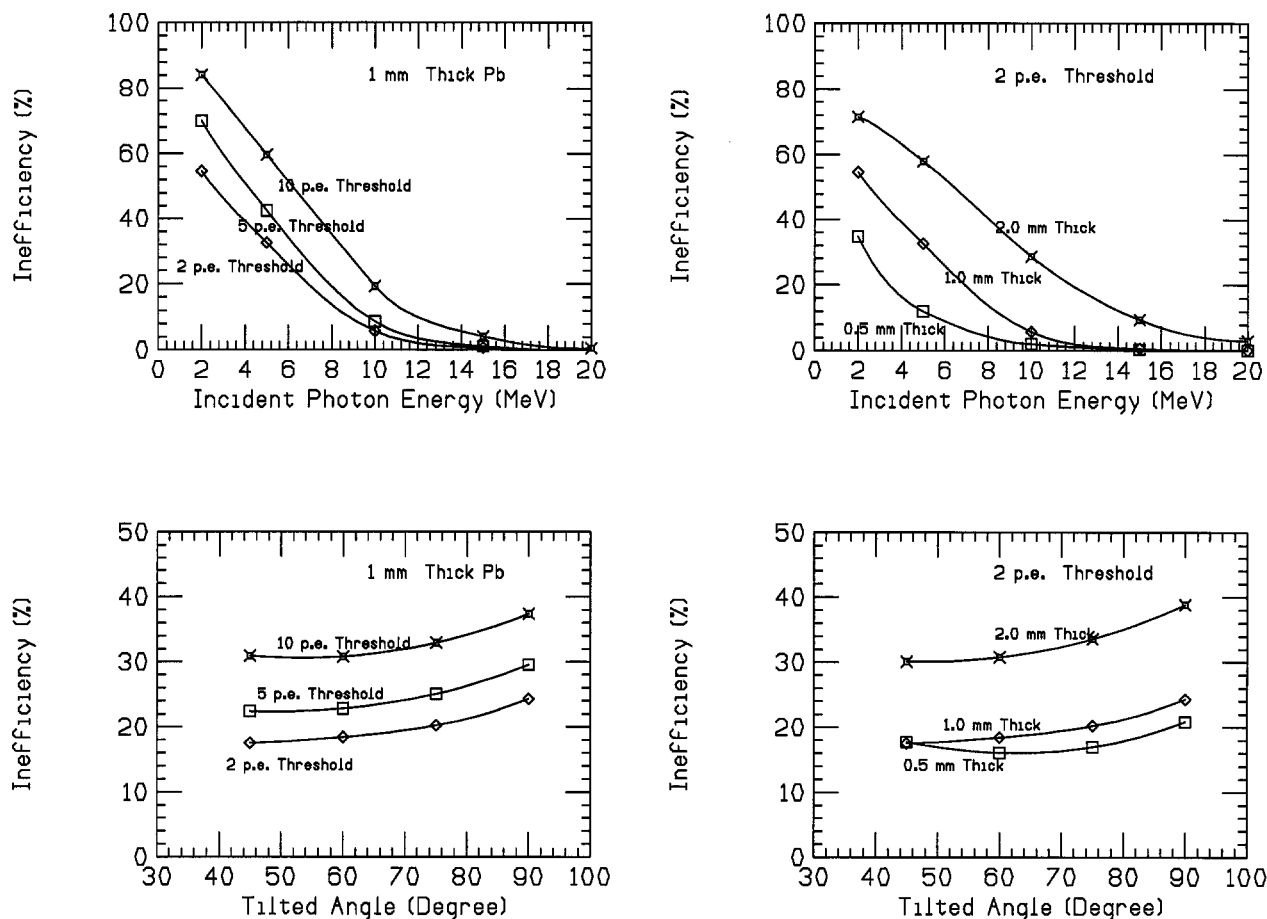
Figure 19: Photon detection inefficiency in the vacuum veto counters. The top two plots show the inefficiency as a function of photon energy, for various photo electron thresholds and lead sheet thicknesses. The bottom two plots show the average inefficiency for photons below 20 MeV as a function of the lead sheet tilt angle.
