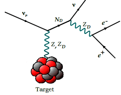
FIG. 1. Contributions to the cross section that in our model gives rise to MiniBooNE's excess of electron-like events.
