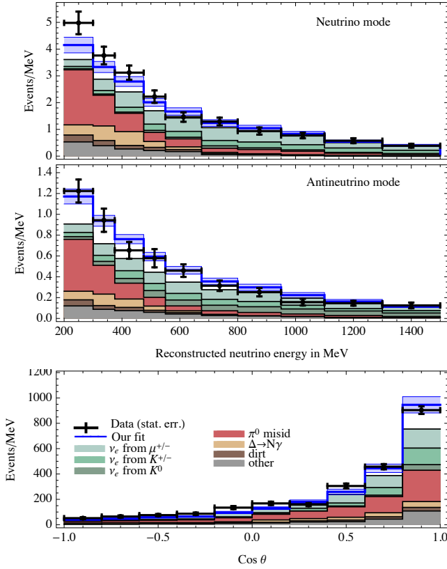
FIG. 2. The MiniBooNE electron-like event data [18] in the neutrino (top panel) and antineutrino (middle panel) modes as a function of E_{\nu}^{\text{rec}} , as well as the \cos \theta distribution (bottom panel) for the neutrino data. Note that the data points have only statistical uncertainties, while the systematic uncertainties from the background are encoded in the light blue band. The predictions of our benchmark point m_{N_D} = 320 MeV, m_{Z_D} = 64 MeV, |U_{\mu 4}|^2 = 10^{-6} , \alpha_D = 0.25 and \alpha \epsilon^2 = 3 \times 10^{-9} are also shown as the blue lines.
