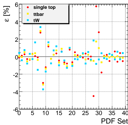
Figure 6.8: Relative variation (in %) of the selection efficiencies for signal, t\bar{t} , and tW , versus the PDF-set index in the CTEQ61 collection. [125]
