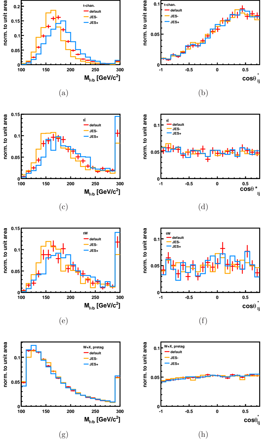
Figure 6.12: Shape comparisons for the invariant top-quark mass M_{l\nu b} (left column) and the restricted \cos\theta_{lj}^* (right column) for a variation of the jet energy scale , for signal ((a), (b)), t\bar{t} ((c), (d)), tW ((e), (f)), and W+X ((g), (h)). The shapes of the top-quark processes are extracted from the sample having passed the standard selection, while the W+X shapes are obtained from pretag samples, where no b -tagging was applied in order to increase the number of events.
