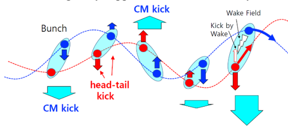
Figure 2: Schematic figure of centre of mass (CM) kick of a bunch-by-bunch TF and head-tail kick. [Courtesy of Nakamura]
