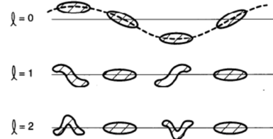
Figure 1: This figure shows longitudinal modes of head-tail instability. l = 0 is the dipole mode and l = 1, 2 are next higher modes.
