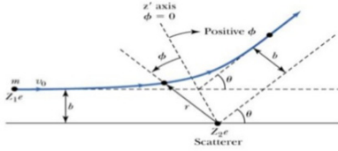
Figure 4: Schematic figure of general Rutherford scattering. In this figure, the incoming particles are positively charged whereas they are electrons in this paper. But, \theta has the same magnitude just with negative sign.
