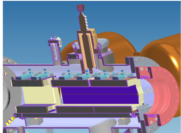
Figure 1: Cross section of the vacuum assembly design.
