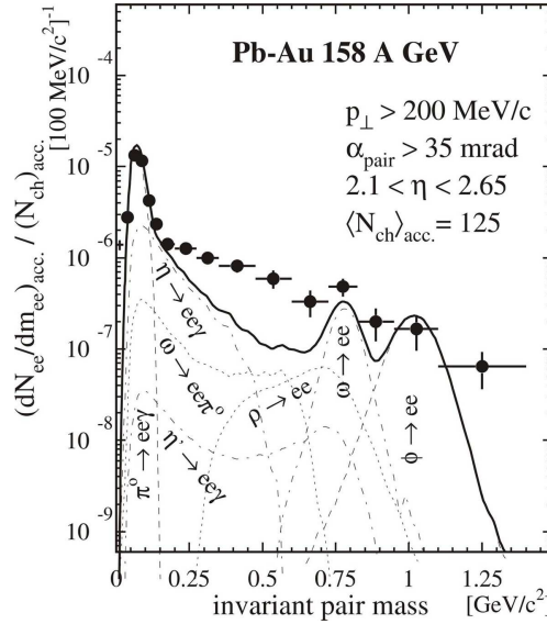
Fig. 1. CERES dielectron invariant mass distribution from 158 A GeV Pb + Au collisions [2] at the CERN SPS. The data is compared to the signal expected from known hadronic sources measured in p+Be collisions (solid line). A large excess in the mass region below the omega meson mass is observed which can only partially be attributed to pion annihilation which is not present in the hadronic cocktail.
