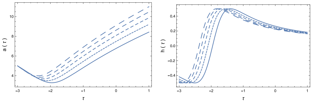
Fig. 6 Time evolution of the scale factor a (left figure) and of the dimensionless Hubble function h (right figure) in a loop quantum cosmological Universe filled with a deformed photon gas satisfying the dispersion relation E = kc\sqrt{1 - 2\beta k^2} , for different values of the parameter A_3 : A_3 = 4 \times 10^{-44} (solid curve), A_3 = 5 \times 10^{-44} (dotted
