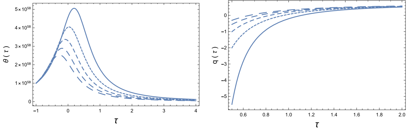
Fig. 10 Time evolution of the dimensionless temperature \theta (left figure) and of the deceleration parameter q (right figure) in a loop quantum cosmological Universe filled with a deformed photon gas satisfying the dispersion relation E = kc(1 - \alpha k) , for different values of the parameter A_4 : A_4 = 4 \times 10^{-58} (solid curve), A_4 = 5 \times 10^{-58} (dotted
