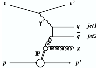
Fig. 14. Diagram describing diffractive production of a q\bar{q}g state in the diffractive structure function approach.
