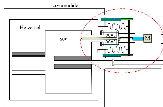
Figure 2: Overview of the plunger tuner with cavity.
