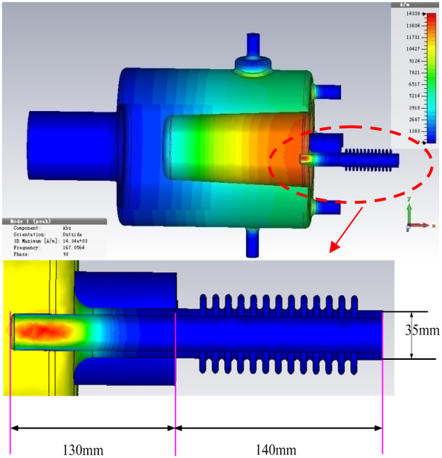
Figure 6: The simulation mode of plunger tuner with cavity.
