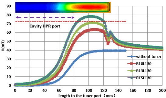
Figure 5: Magnetic field along the plunger for three plunger radii.
