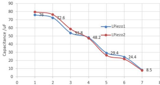
(a) Capacitance varies during cooling down of high voltage Piezo.
