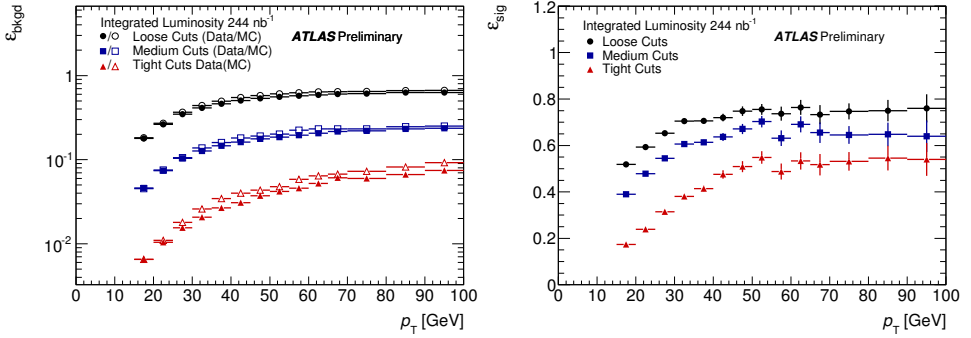
Fig. 3. Background efficiencies obtained from di-jet data and MC samples as a function of the reconstructed p_T^\tau (left). Signal efficiencies obtained from Z \rightarrow \tau\tau MC sample as a function of the reconstructed visible p_T^\tau (right).
