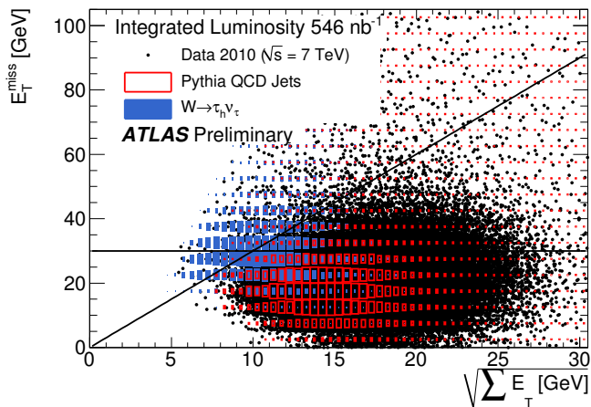
Fig. 5. Distribution of events in the E_T^{\text{miss}} vs. \sqrt{\sum E_T} plane after the trigger requirement for data, simulated signal events and QCD background. The applied E_T^{\text{miss}} and E_T^{\text{miss}} significance cuts are indicated as solid lines.
