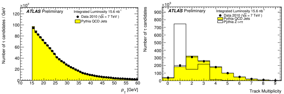
Fig. 2. Transverse momentum distribution (left) and number of associated tracks of \tau candidates (right). The number of \tau candidates in MC samples are normalised to the number of \tau candidates selected in data. The data correspond to an integrated luminosity of 15.6 \text{ nb}^{-1} .
