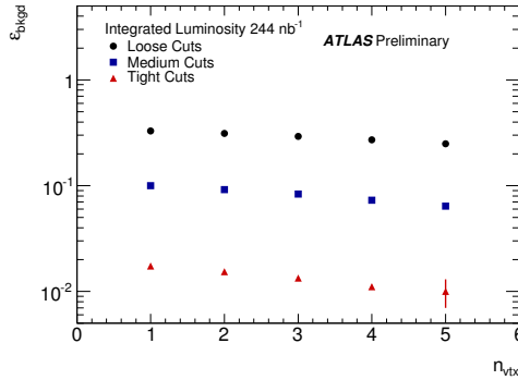
Fig. 4. Background efficiencies as a function of number of vertices n_{vtx} .
