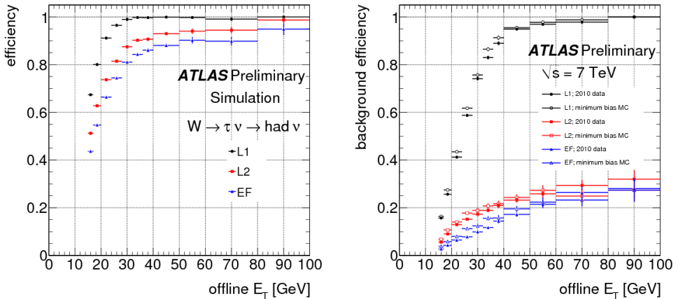
Fig. 1. Fraction of reconstructed tau candidates (no identification applied) passing L1 ( p_T > 5 GeV), L2 ( p_T > 7 GeV) and EF ( p_T > 12 GeV) loose trigger conditions as a function of E_T of the offline candidate. Left: signal efficiency on W \rightarrow \tau\nu ; right: data-MC comparison on minimum bias background.
