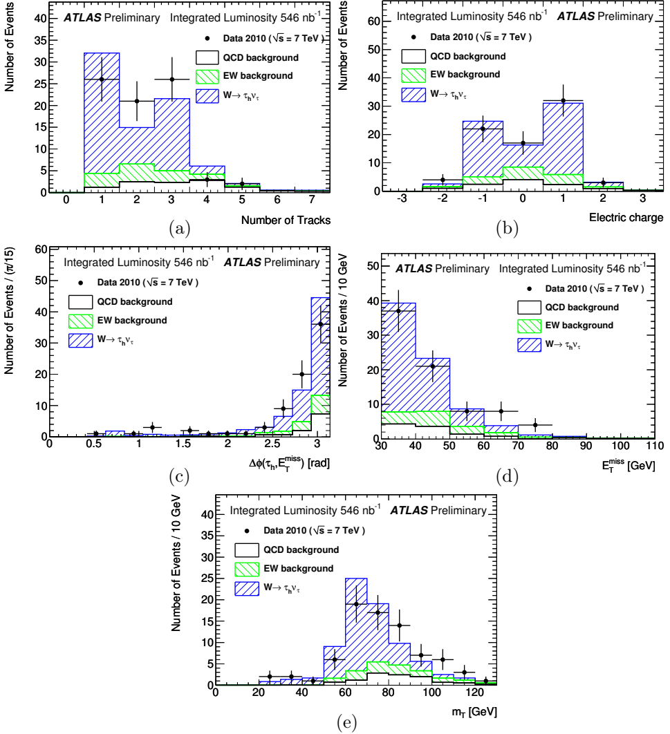
Fig. 6. Distributions of the tau track multiplicity (a), electric charge (b), \Delta\phi(\tau_h, E_T^{\text{miss}}) (c), E_T^{\text{miss}} (d) and transverse mass m_T (e) for the data in signal region A, the scaled QCD background from control region C, and the contributions from signal and EW background in region A. The QCD background distribution is normalized to the estimated number of QCD background events in region A ( N_{\text{QCD}}^A ).
