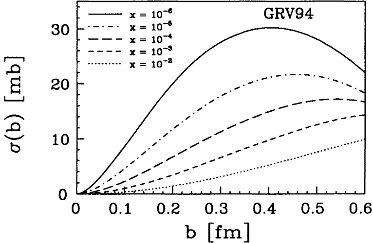
Fig. 1. Colour-dipole cross section, \sigma_{q\bar{q}N}(x, b) of Eq. (3), as a function of the transverse size of the q\bar{q} pair for various values of x and for the GRV94 parameterization of the nucleon's gluon density.
