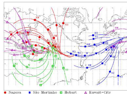
Fig. 3: The complete coverage of the GMDN - Global Muon Detector Network with the directions for each MMD's: Nagoya, Japan 17 directions; Hobart, Australia 13; Kuwait, Kuwait 13; So Martinho da Serra, RS, Brazil 17 (V, N, S, E, W, NE, NW, SE, SW, N2, S2, E2, W2, N3, S3, E3, W3).
