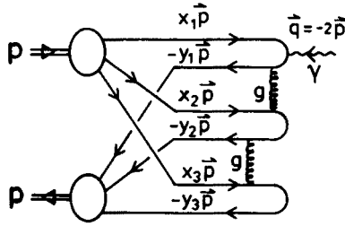
Fig. 9. Lowest order hard-gluon exchange needed to turn over the spectator quarks in the nucleon, viewed in the Breit frame.
