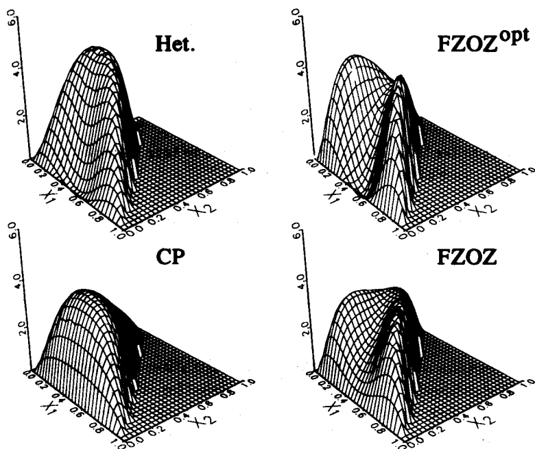
Fig. 8. Profiles of model distribution amplitudes for the \Delta^+ -isobar, derived from QCD sum rules.
