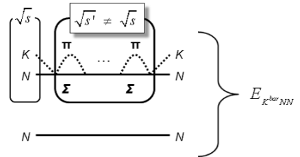
Fig. 1. Diagrammatic explanation of the effective \bar{K}N potential used in DHW (left panel) and three-body \pi\Sigma N dynamics (right panel).
