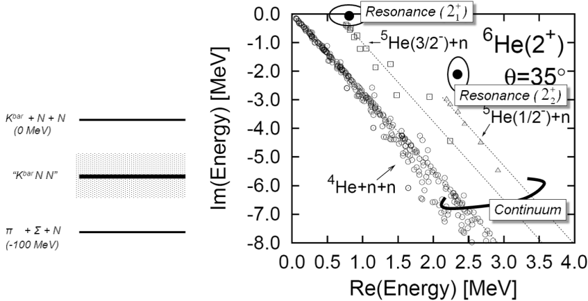
Fig. 2. (Left) Threshold relation. (Right) Result of {}^6\text{He} calculated with CSM at \theta = 35^\circ . (Given by Dr. Myo [11].)
