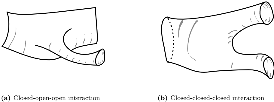
Figure 1.1: Two of the possible interactions of the string. The left panel depicts the emission of a closed string from two open ones, while the right panel features three closed strings. Notice that there is no localised interaction vertex.
