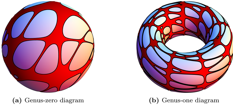
Figure 1.3: The order in 1/N of a diagram is given by the genus of the simplest surface where it can be drawn without self-intersections. In panel (a), we can draw a ribbon graph on a sphere (genus zero), while in panel (b) we draw one on a torus (genus one). Note that these ribbon graphs have a large number of vertices and approximate well a smooth surface—a qualitative similarity between ribbon graphs and the string worldsheet.
