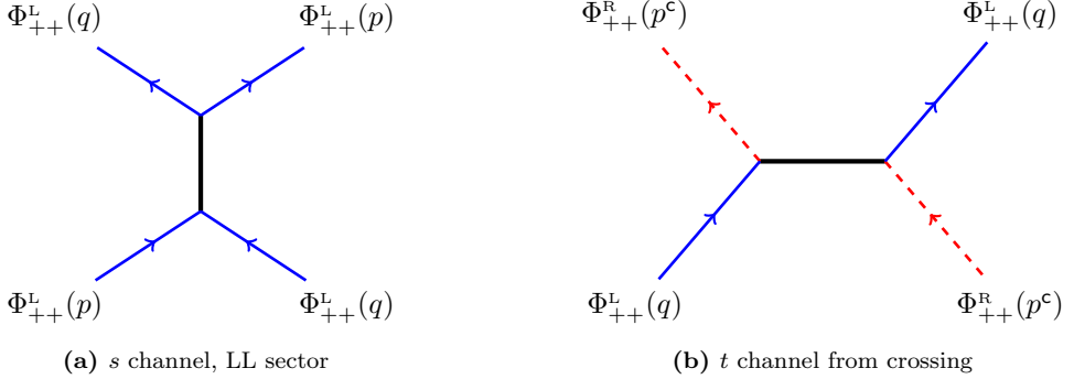
Figure 4.4: On the left two particles in the same sector form an \mathfrak{su}(2) bound state in the s channel. Applying the crossing transformation to \Phi_{++}^L(p) yields the t -channel diagram on the right, where one particle has unphysical momentum p^c (red dashed lines).
