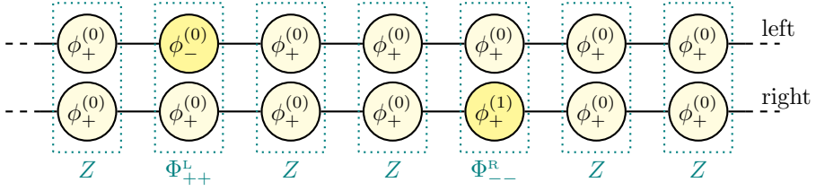
Figure 5.3: A pictorial representation of the \mathfrak{psu}(1,1|2)^2 spin chain. We can think of it as two (left and right) spin chains, each with ground state \phi_+^{(0)} . Excitations of the whole chain are considered as left- or right- moving depending on whether we excite a spin in the left or right chain.
