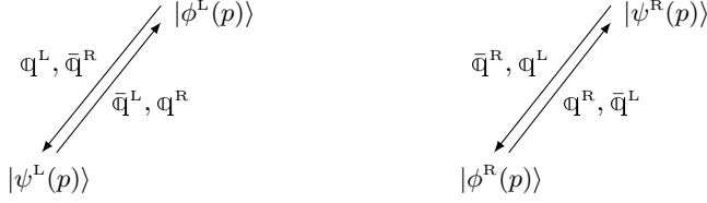
Figure 2.3: The action of the supercharges q^{L,R} and \bar{q}^{L,R} of \mathfrak{psu}(1|1)_L \oplus \mathfrak{psu}(1|1)_R centrally extended on an arbitrary momentum (off-shell) excitation (2.102).
