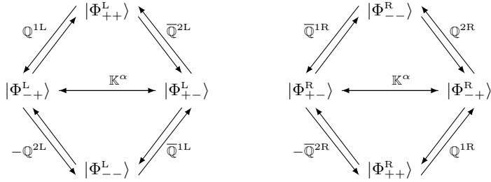
Figure 8.1: The action of the supercharges on the massive excitations is supplemented by \mathbb{K}^\alpha from \mathfrak{su}(2)_K , acting on the fermions. Note that for clarity we only depict the action of some of the supercharges, i.e. the ones that remain non-trivial on-shell.
