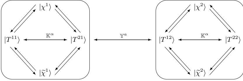
Figure 8.2: The massless excitations sit in two \mathfrak{psu}(1|1)_{\text{c.e.}}^4 modules, with fermionic highest weight states. The two modules transform as a doublet under \mathfrak{su}(2)_Y , and additionally the bosons T^{\alpha a} also carry a Greek index of \mathfrak{su}(2)_K .
