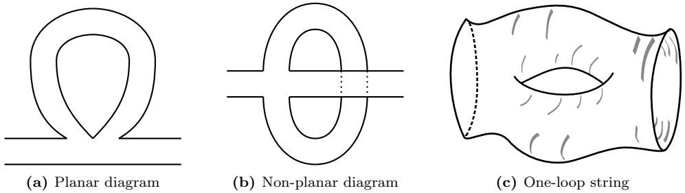
Figure 1.2: Diagrammatic expansions in terms of the topology of the graphs. The first two panels exemplify the perturbation theory of Yang-Mills theories in terms of ribbon graphs. Panel (a) depicts a one-loop contribution to the two-point function that is planar, while the contribution in panel (b) cannot be drawn on a plane without self-intersections, and is subleading in a 1/N expansion. In panel (c), the genus expansion also appears naturally for closed strings, due to the interactions of figure 1.1b.
