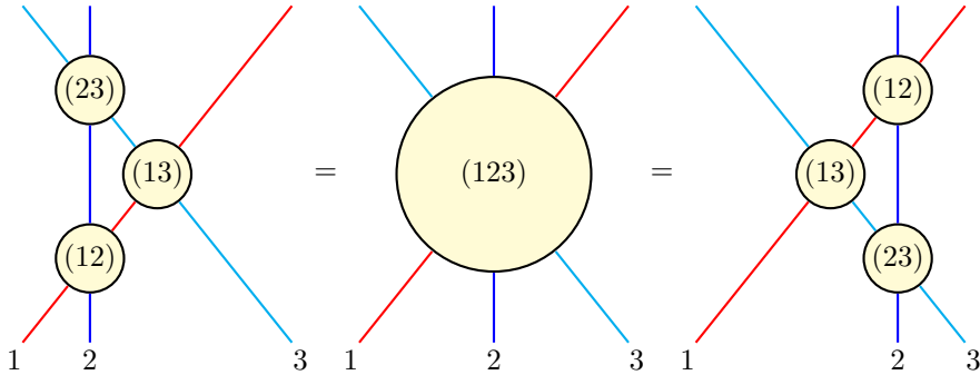
Figure 3.2: Different ways of resolving the 3 \rightarrow 3 particle scattering (central panel). Taking time to flow upwards, we have in the left panel the sequence of scattering (12)-(13)-(23), while in the right panel we have (23)-(13)-(12). The Yang-Baxter equation imposes the equality of the two resolutions.
