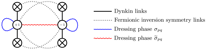
Figure 6.4: The Dynkin diagram for \mathfrak{psu}(1,1|2)^2 with the various interaction terms appearing in the Bethe ansatz indicated. The label \pm 1 inside the middle Dynkin nodes indicate the \mathfrak{su}(2) and \mathfrak{sl}(2) gradings of the left- and right-moving sectors.
