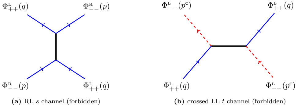
Figure 4.5: On the left the would-be Landau diagram for one left- and one right-moving particle is depicted. This process should be absent. Similarly, the crossed process on the right should be absent, and the corresponding S-matrix element have no pole.
