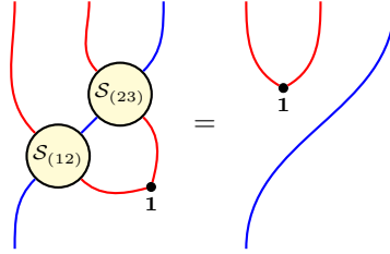
Figure 5.5: The scattering of a fundamental excitation with a singlet is trivial. We depict the singlet as composed of two excitations, one of which moves “backward” due to analytical continuation to the crossed region.
