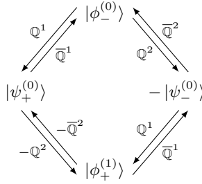
Figure 5.2: The action of the supercharges Q^j = Q^{jL,R} and \bar{Q}^j = \bar{Q}^{jL,R} on either of the left- or right-bifundamental representation (5.17). It takes the same form of figure 2.2.
