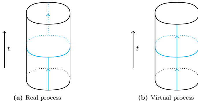
Figure 1.4: Two processes involving exchange of real or virtual particles that wrap around the worldsheet cylinder, and therefore are not captured by the Bethe-Yang equations.
