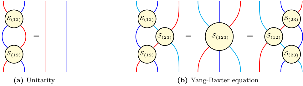
Figure 5.4: Consistency conditions on the spin-chain S matrix. Unitarity (left panel) requires that acting twice with S_{(12)} on a two-particle state gives back the original state. The Yang-Baxter equation (right panel) resolves the ambiguity in decomposing the scattering of three excitations. Note how, with respect to figure 3.2, this picture takes into account how S permutes the spin-chain excitations.
