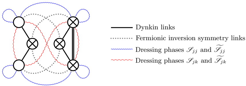
Figure 8.5: The Dynkin diagram for \mathfrak{d}(2,1;\alpha)^2 in mixed grading (see figure 8.3), with the various interaction terms of the Bethe ansatz indicated. Note how now, besides dressing phases that couple nodes of the same mass (in blue), there appear phases coupling nodes of mass \alpha with ones of mass 1 - \alpha (in red).
