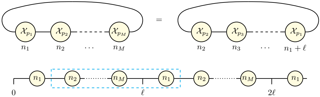
Figure 6.1: Illustrations of the periodicity condition leading to the Bethe ansatz equations. Above: the two ends of the chain have been identified, so that the first excitation \mathcal{X}_{p_1} in position n_1 can be thought as sitting at the end of the chain, in position n_1 + \ell . This can be realised by scattering \mathcal{X}_{p_1} through all of the \mathcal{X}_{p_j} . Below: equivalently, the wave-function should be \ell -periodic as a function on \mathbb{R} . The box identifies the periodicity condition evaluated as in (6.5).
