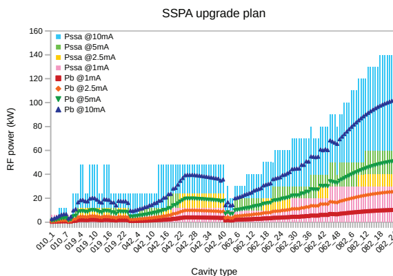
Figure 3: SSPA group utilization.
