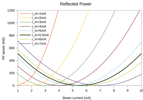
Figure 2: Reflected RF power ratio at different P_{b,m} .
