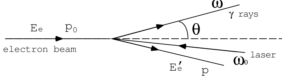
Fig. 1. Backscattered Compton Process via the collision between high energy electron and laser light.
