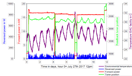
Figure 3: The forward, reflected powers vs. temperature while the sliding mode control implemented.
