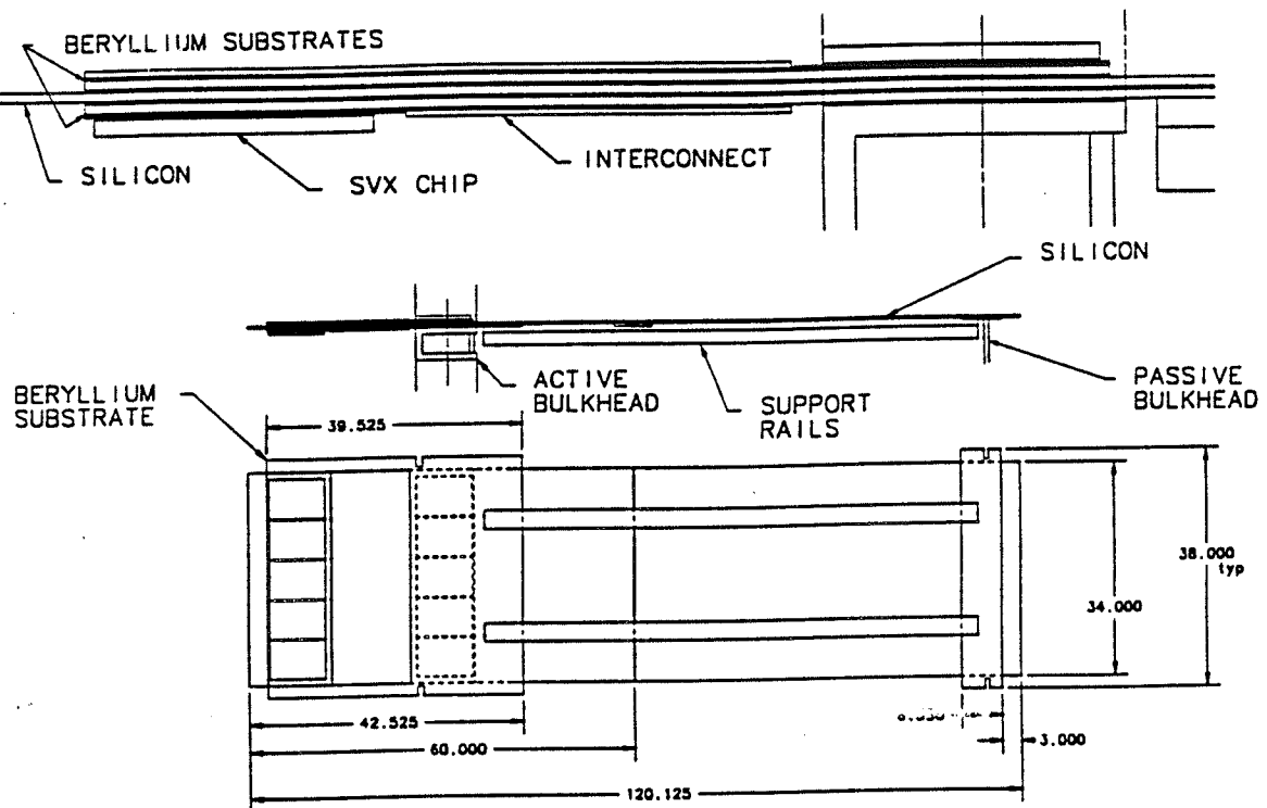
Fig. 2. Five-chip-wide ladder.
