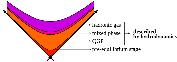
Fig. 1. Description of QGP formation in heavy ion collisions. The kinematic landscape is defined by \tau = \sqrt{x_0^2 - x_1^2} ; \eta = \frac{1}{2} \log \frac{x_0 + x_1}{x_0 - x_1} ; x_T = \{x_2, x_3\} , where the coordinates along the light-cone are x_0 \pm x_1 , the transverse ones are \{x_2, x_3\} and \tau is the proper time, \eta the “space-time rapidity”.
