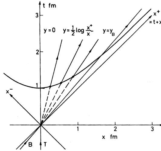
Fig. 2. In-Out cascade. The “piece of fluid” with space-time rapidity \eta gives rise to hadrons at rapidity y \equiv \eta , after crossing the “freeze-out” hyperbola at fixed proper-time \tau .
