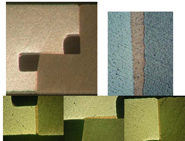
Figure 2 : Micrographs of Joint A. The stainless steel mating part is the lighter shade and the Niobium part is the darker shade. The two grooves for the filler material were machined on the stainless steel part (top left). The copper filler material can be seen between the mating parts.
