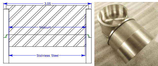
Figure 4 : A sketch (left) and a picture (right) for the trial pieces with expansion plugs installed.
