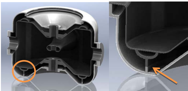
Figure 1 : Sectioned model of the SSR1 resonator (left) and a detail of the coupling ring (right) joining the niobium cavity (dark grey) to the steel helium vessel (light grey).
