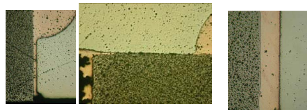
Figure 7 : Micrographs of the large trial pieces showing uniform copper filler material in each of the three areas of the joint.
