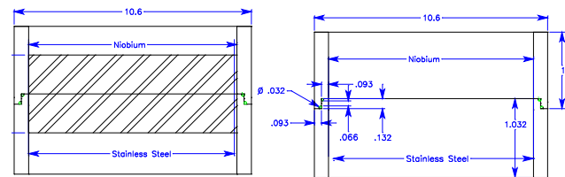
Figure 5 : Geometry of the larger trial pieces. Shown with steel plug (left) and without the plug (right)
